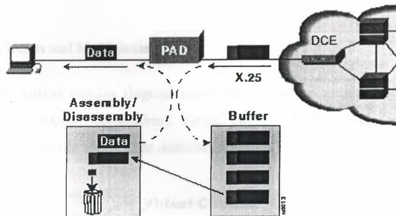
Figure 2.16: Shows the Basic Operation of the PAD
