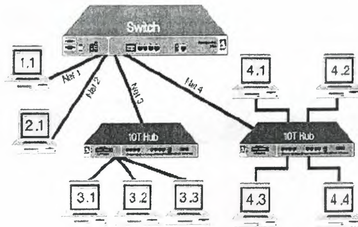
Figure 3.7 Switch connected to Hubs
