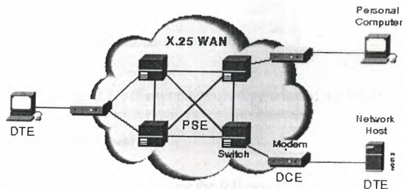
Figure 2.15: Shows the Relationship between X.25 Network Devices
