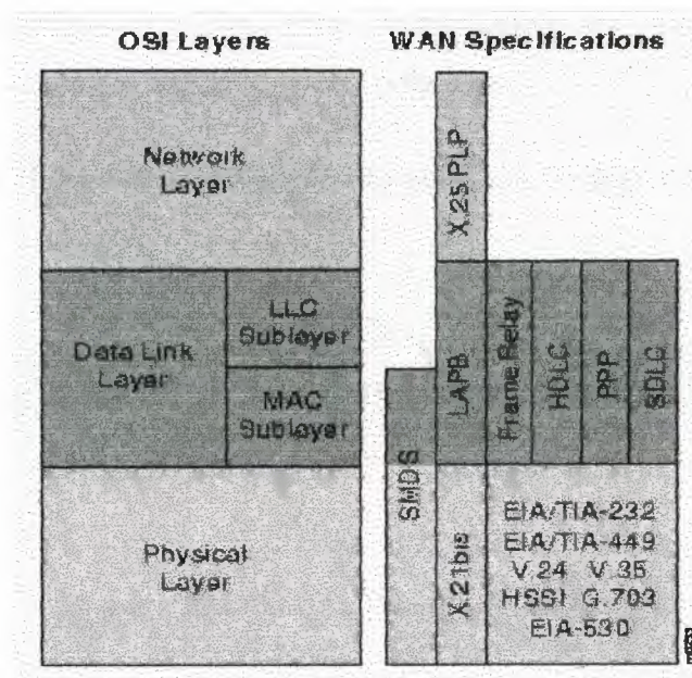
Figure 1.1: Shows WAN Specification and OSI Model
