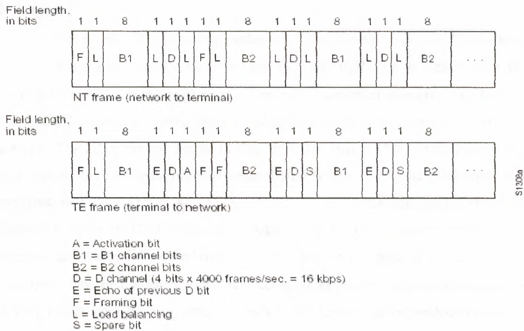
Figure 3.9: Shows ISDN Physical-layer frame formats
