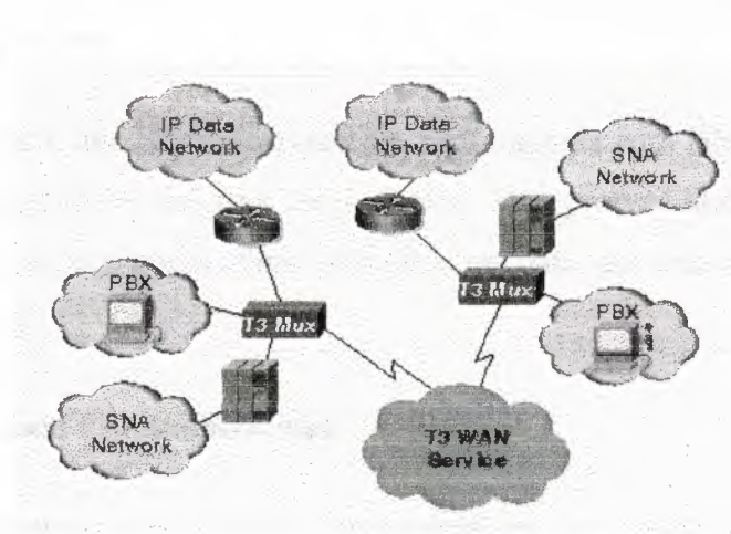
Figure 2.2: Illustrates a Typical HSSI-based T3 WAN
