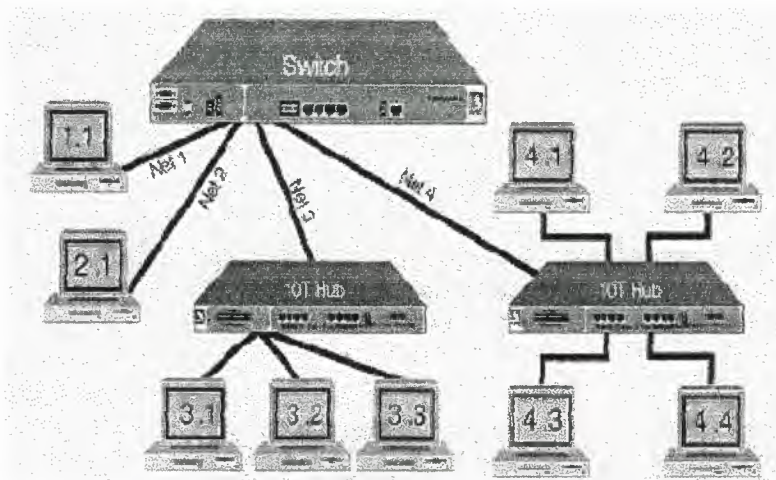
Figure 3.7 Switch connected to Hubs
