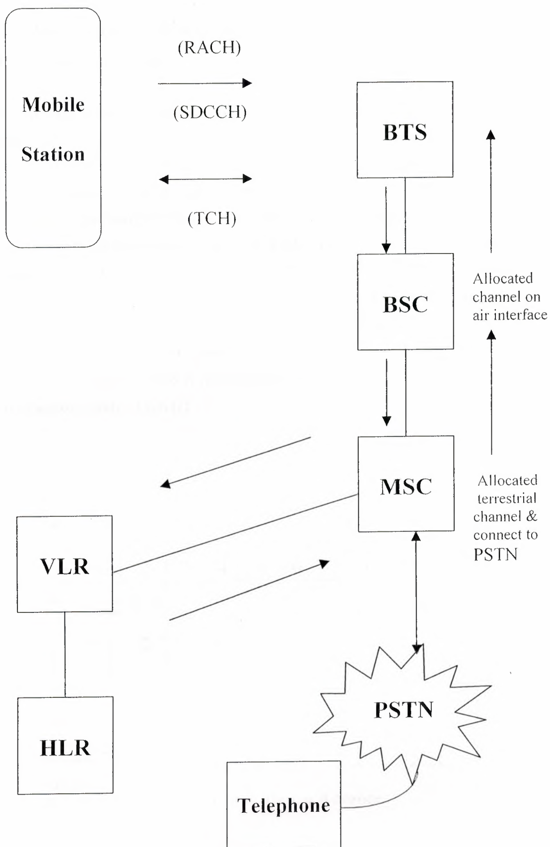
Figure 4.1: GSM Basic Call Sequence
