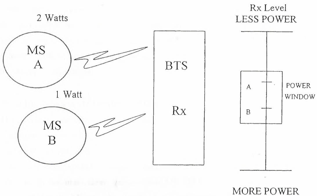
Figure 4.10: Power Control
