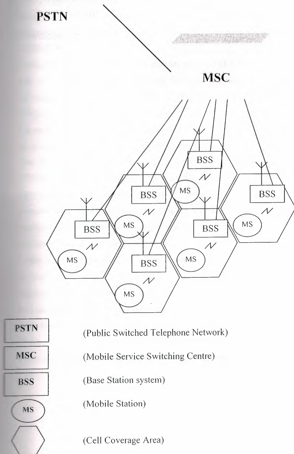
Figure 1.2: Network components
