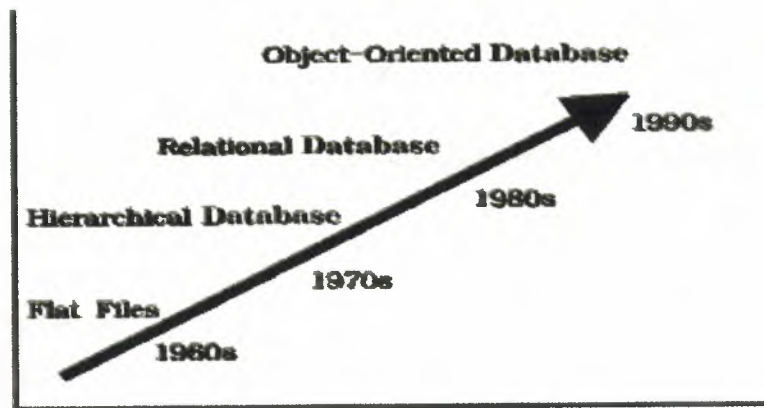
Figure 5.1. Database Trends
