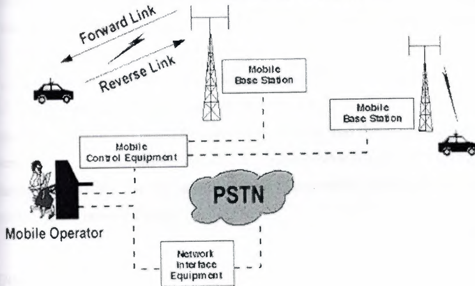
Figure 3.8: Cellular System Components
