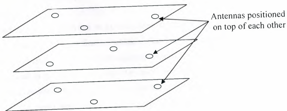
Figure 4.28: Recommended antenna positioning for each consecutive floor, for a building with several indoor cells with very tight re-use.
