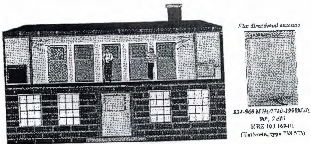
Figure 4.4: Directional antennas.
