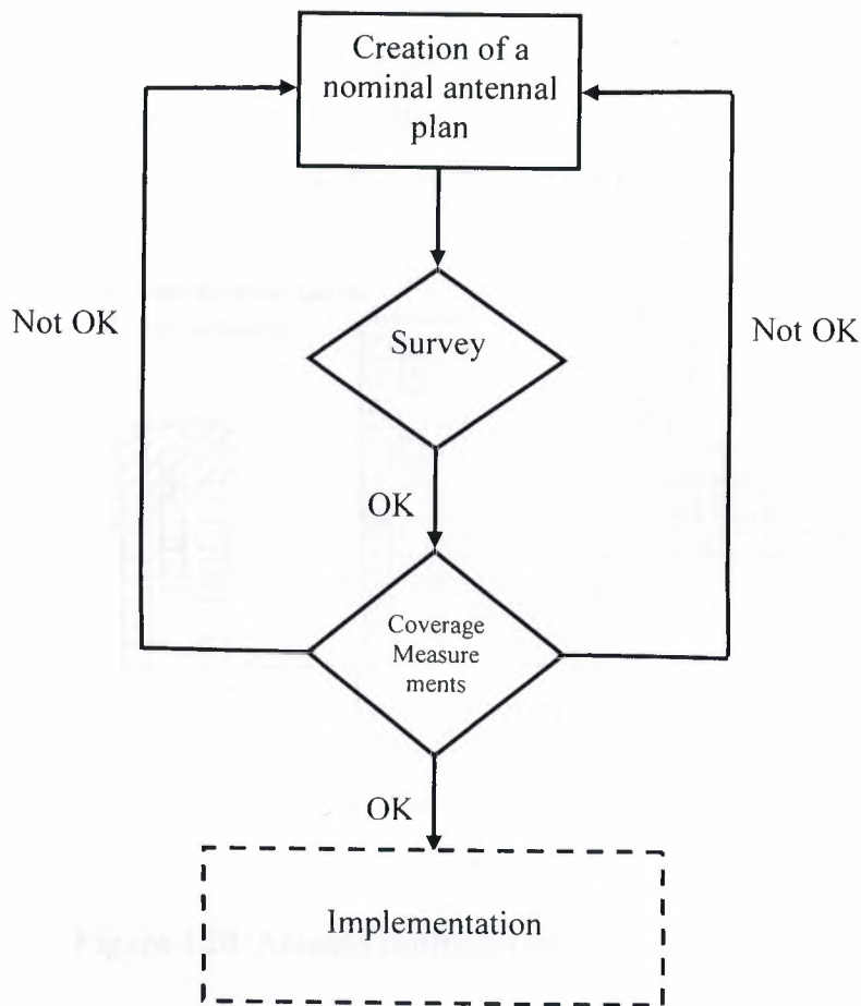
Figure 4.19 Antenna configuration work flow.
