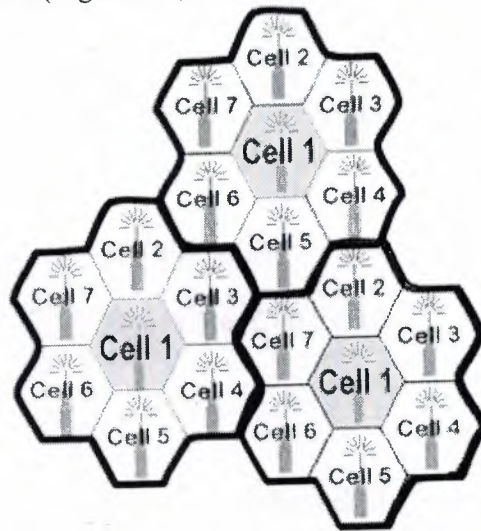
Figure 3.5: Frequency Reuse
