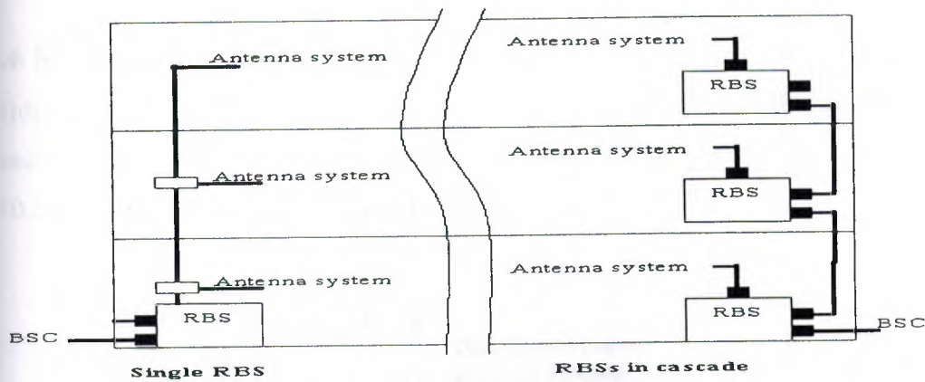
Figure 4.10: BBS configurations
