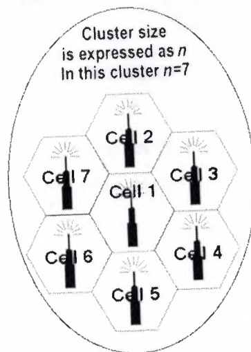
Figure3.4: A Seven-Cell Cluster
