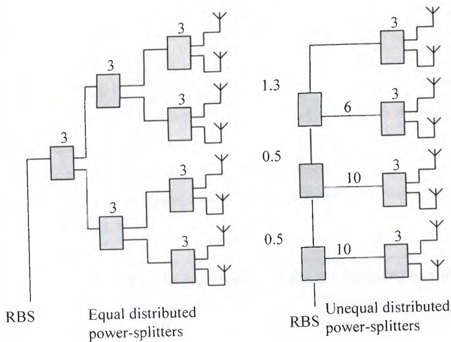
Figure 4.6: Power splitters. Comparison of typical antenna
