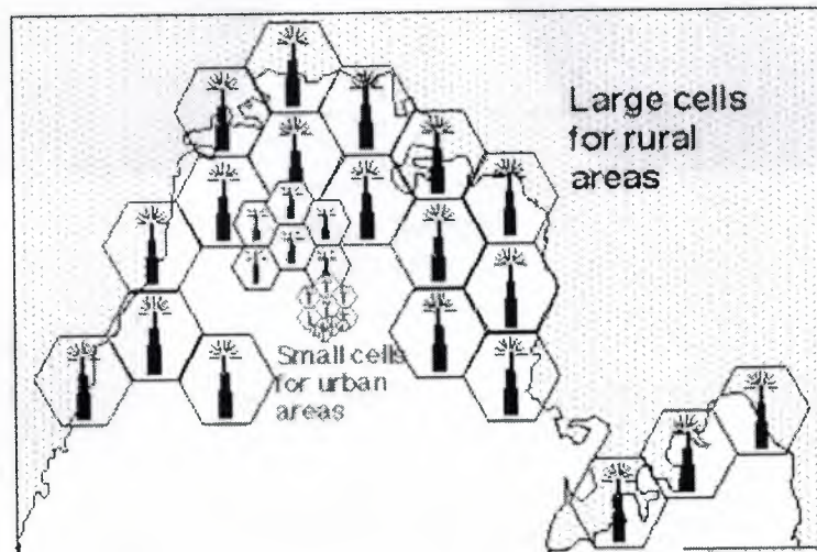
Figure 3.6: Cell Splitting
