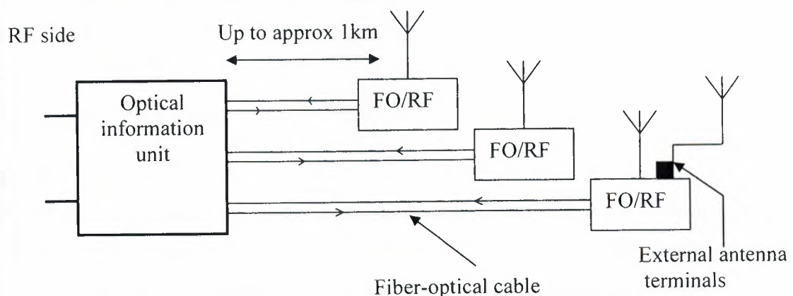
Figure 4.8: Antennas distributed via a fiber-optical network.
