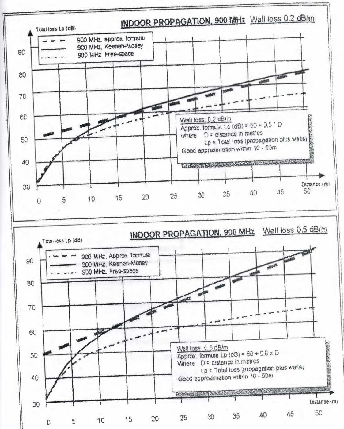
Figure 4.25: diagrams showing approximate indoor propagation loss at 900MHz for a wall Attenuation of 0.2 & 0.5 dB/m. At 1800MHz the loss is 6dB higher.
