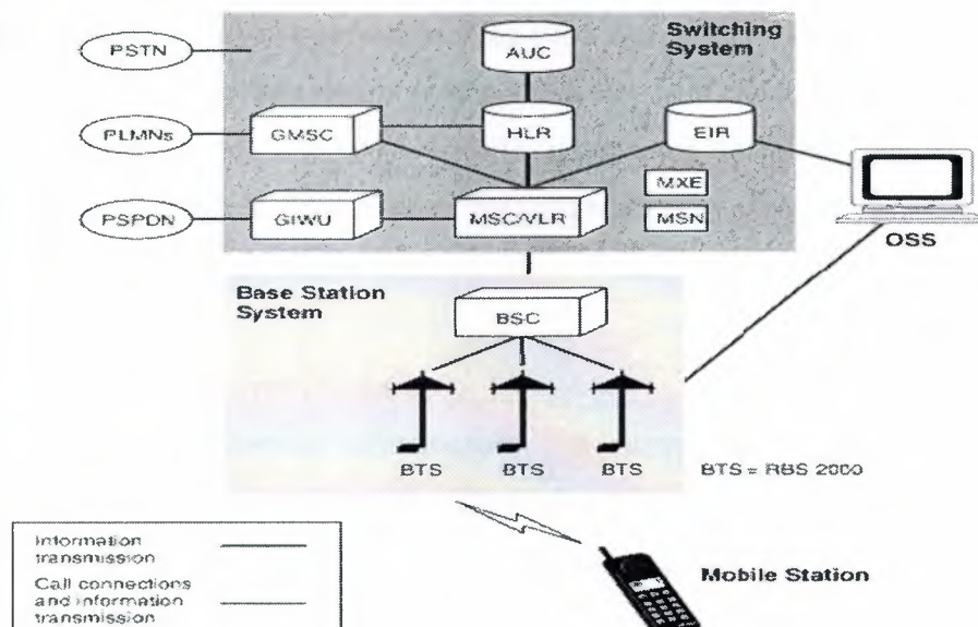
Figure1.1: GSM Network Element
