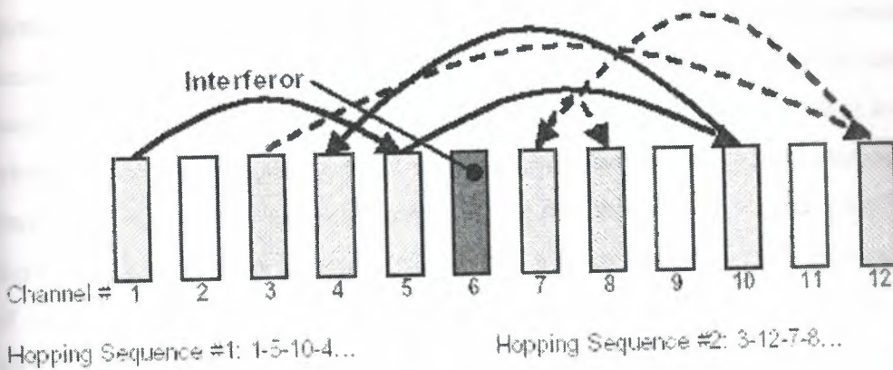
Figure 4.2: Frequency Hopping Spread Spectrum
