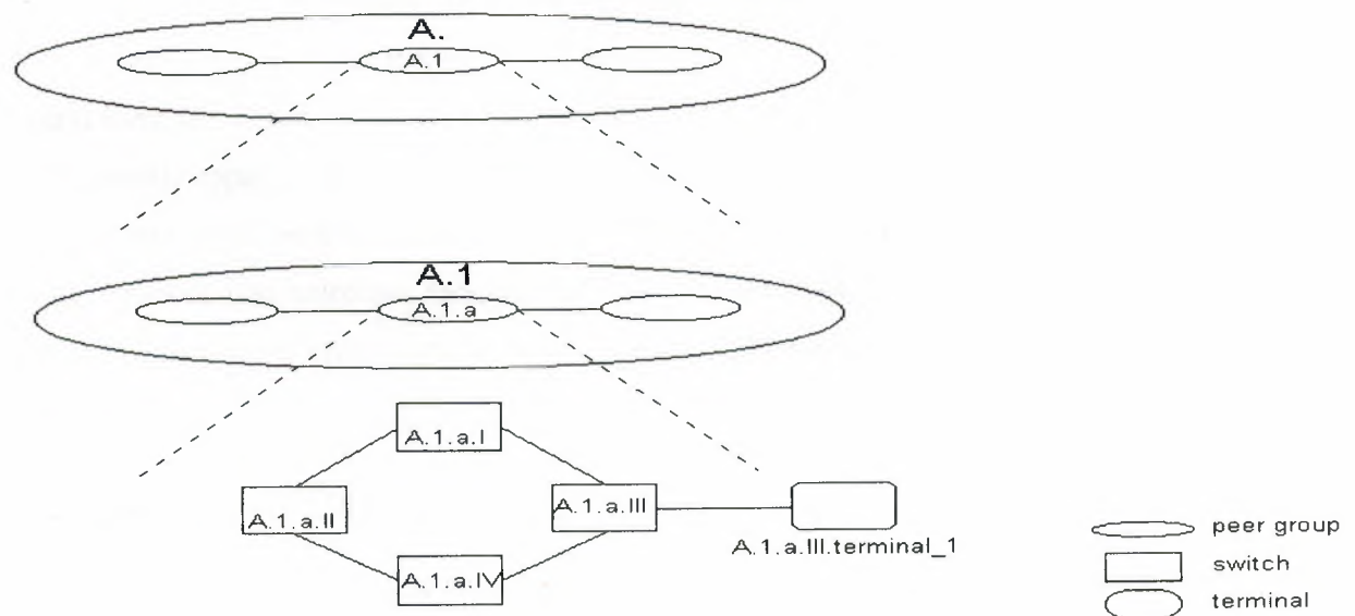
Figure 4.3 An example of a PNNI network
