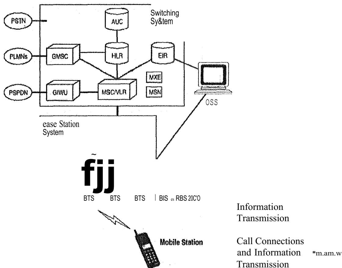
Figure 2.12 GSM Network Elements
