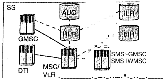
Figure 2.11 Switching System
