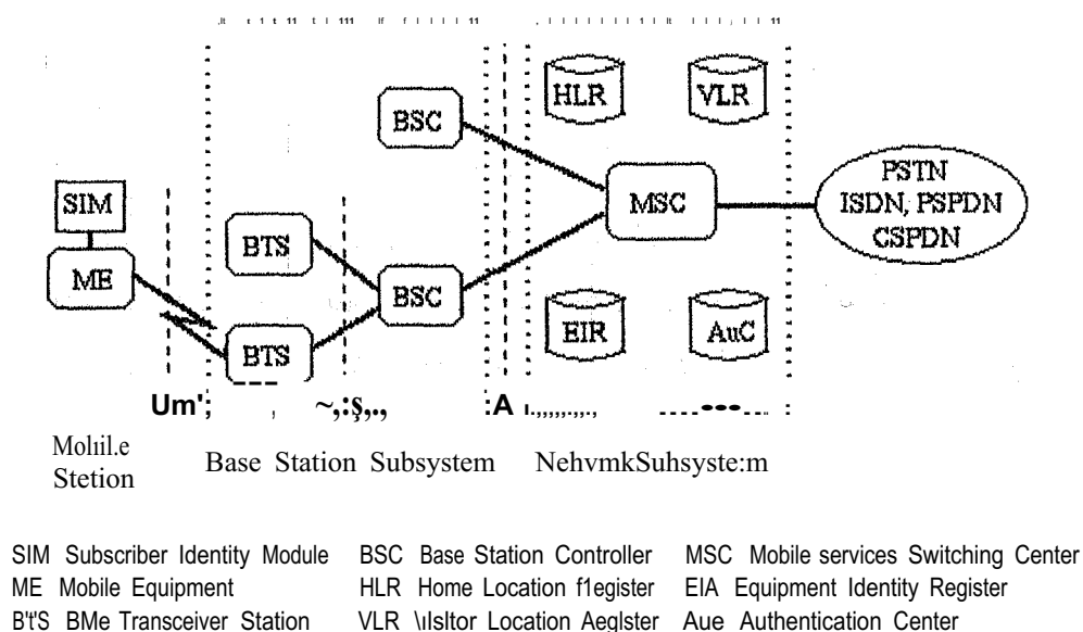
Figure 2.2 General architecture of a GSM network
