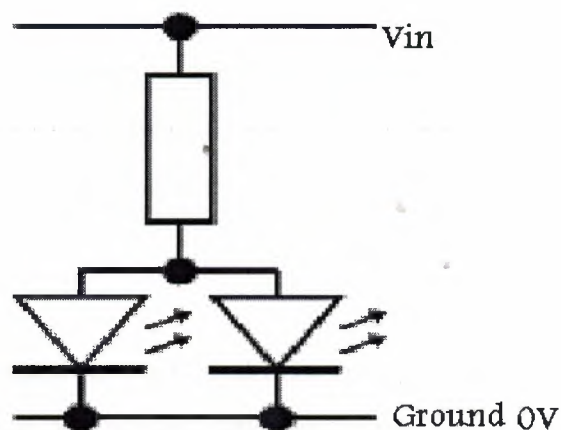
Figure 4.8: Wrong case LEDs connection
