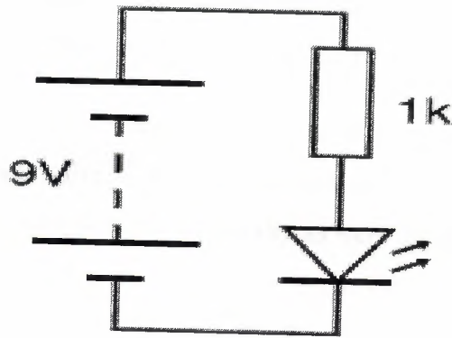
Figure 4.9: A LED connection's diagram
