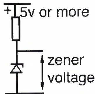
Figure 1.13: Zener diode
