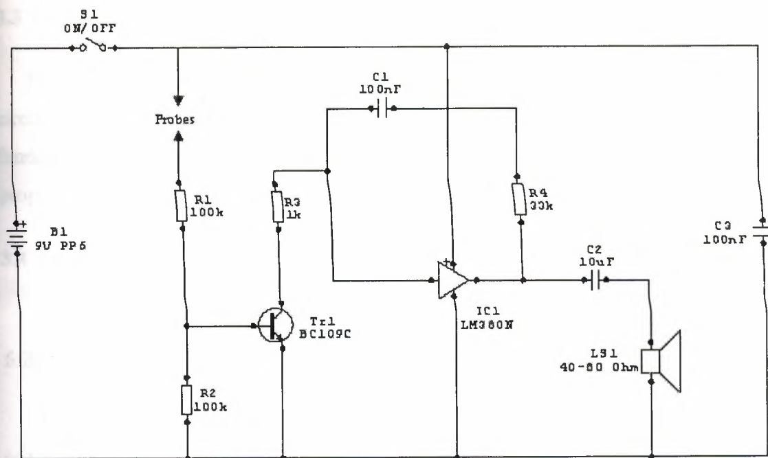
Figure 3.1: Circuit's diagram [19]
