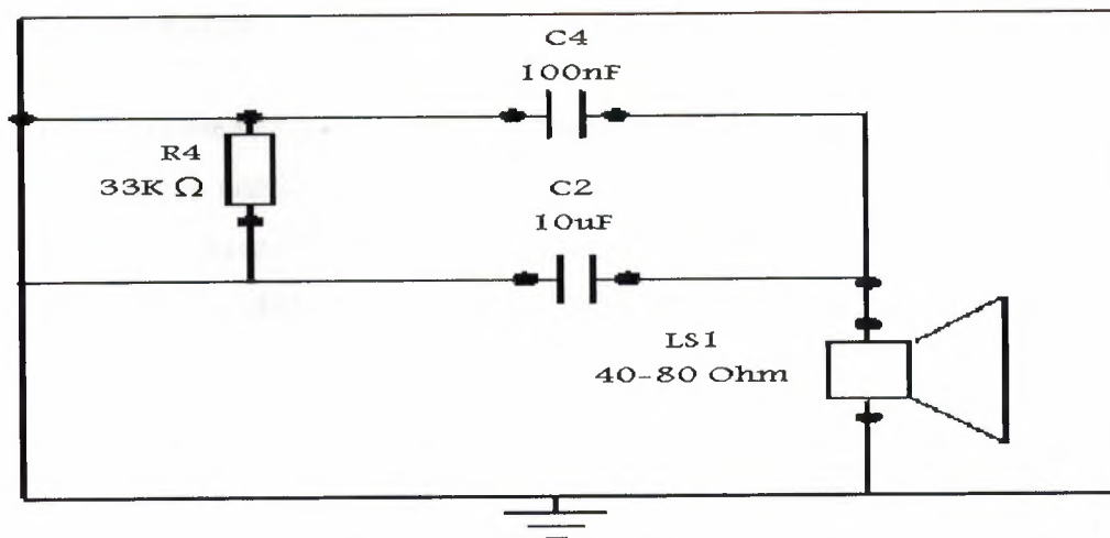
Figure 4.1: Modified portion of the circuit
