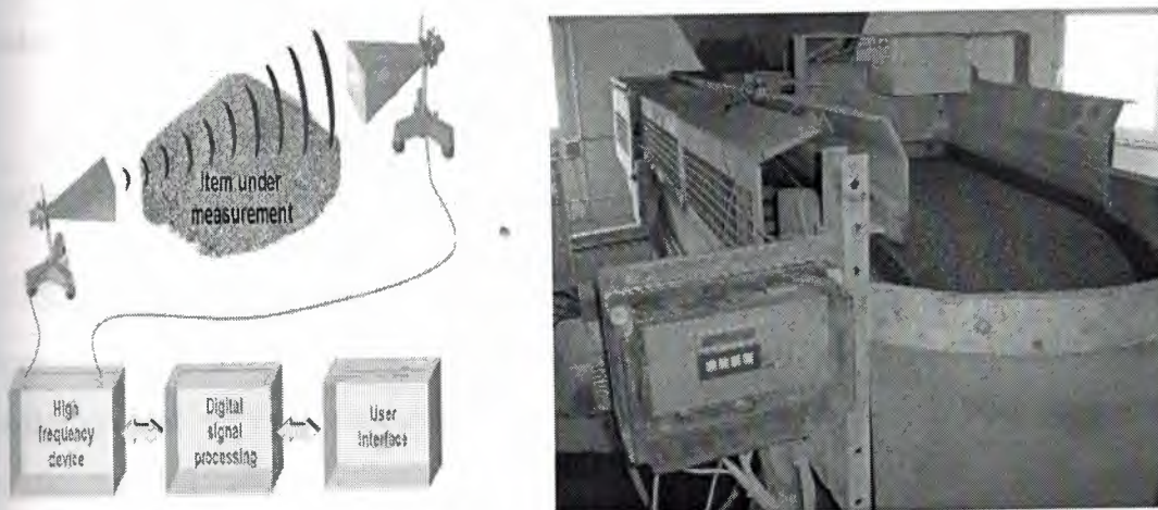
Figure 2.3: Microwaves moisture detector [16]
