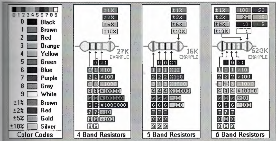
Figure 1.2: Color code identification [4].
