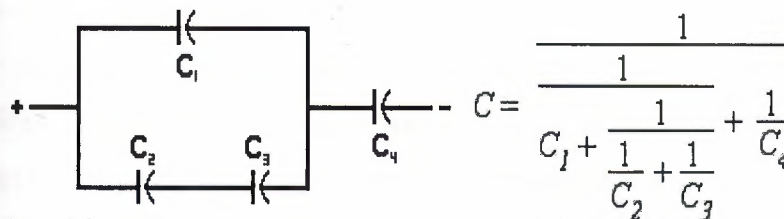
Capacitors in series and parallel
