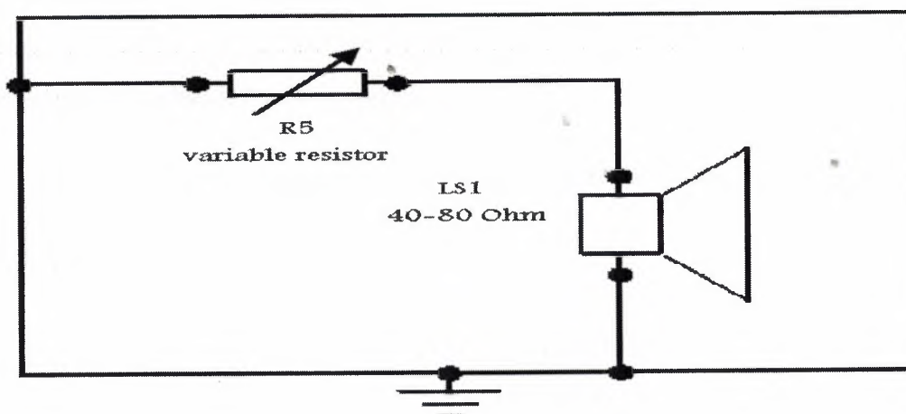
Figure 4.2: Modified portion of the circuit
