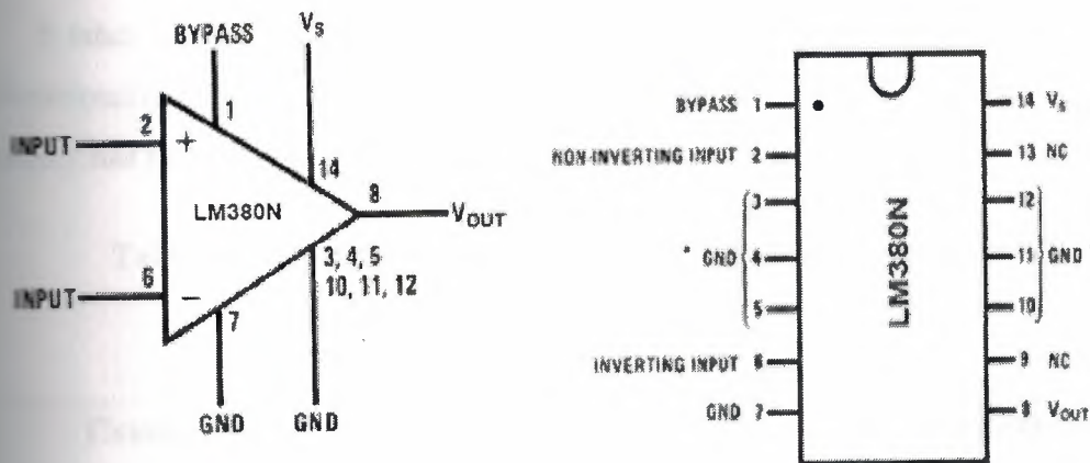
Figure 1.17: IC_LM380N form.
