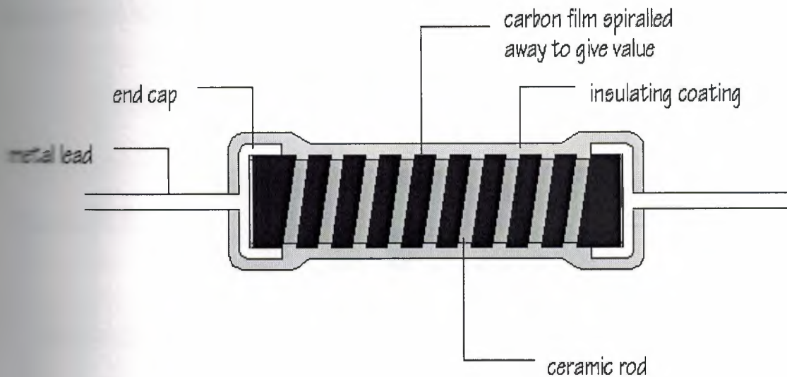
Figure 1.1: The diagram shows the construction of a carbon film resistor [3].
