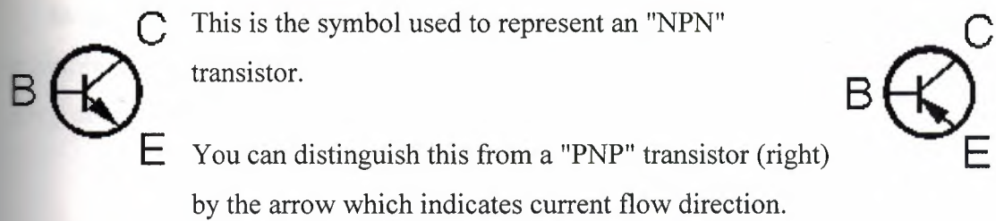
Figure 1.10: The difference between PNP and NPN transistors.
