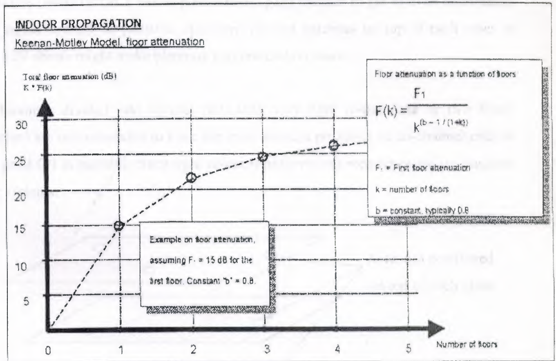
Figure 4.26: loss between floors
