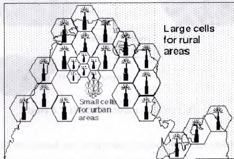
Figure 3.6: Cell Splitting
