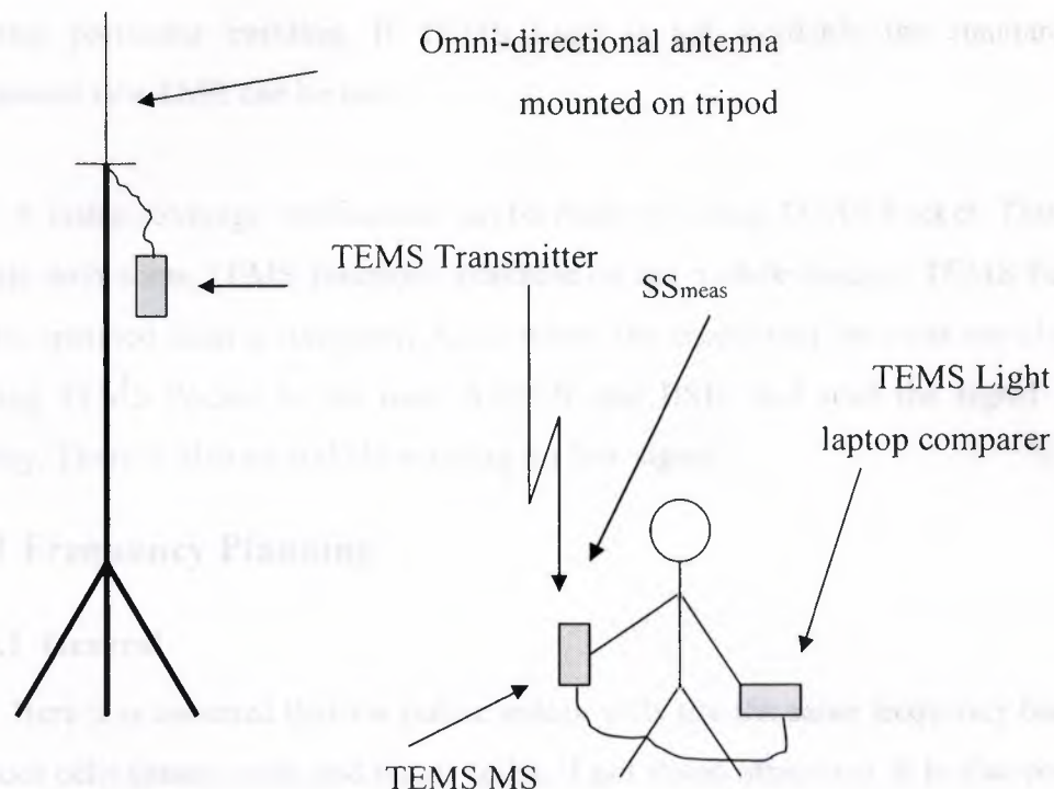
Figure 4.29: Measurement configuration
