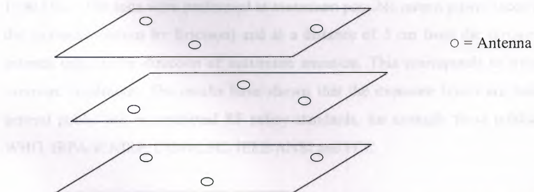
Figure 4.27: Recommended antenna positioning for each consecutive floor for a building with one or several indoor cells.
