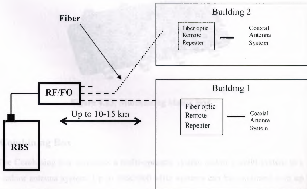
Figure 4.11: Configuration providing coverage at several different locations at large distances.
