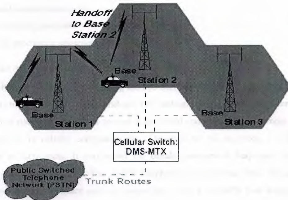
Figure 3.7: Handoff between Adjacent Cells
