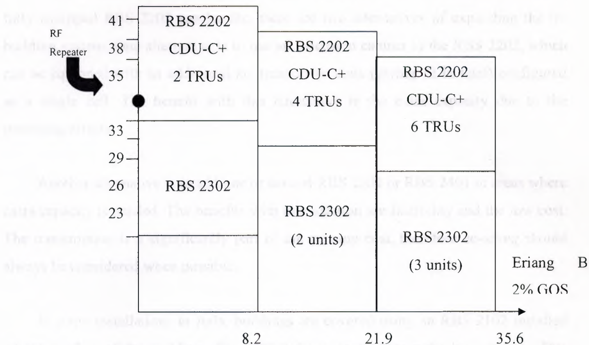
Figure 4.16: Selection of radio unit in a GSM 900 system.
