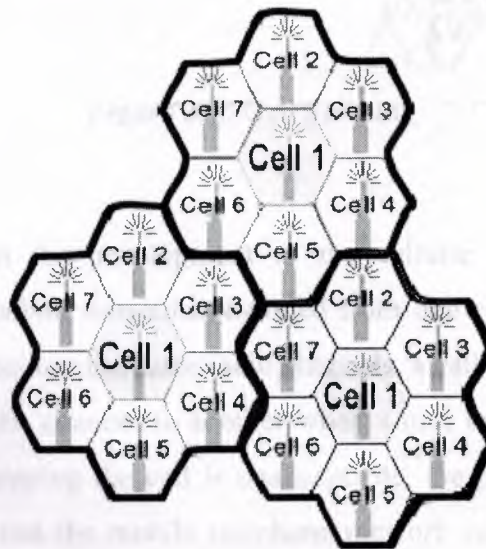
Figure 3.5: Frequency Reuse
