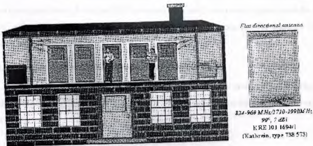
Figure 4.4: Directional antennas.
