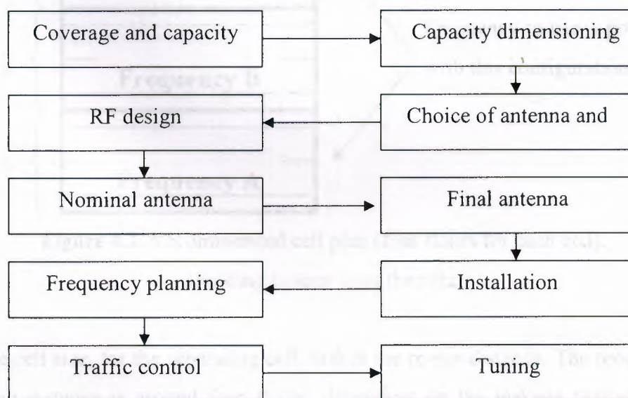
Figure 4.1: The workflow of indoor cell planning
