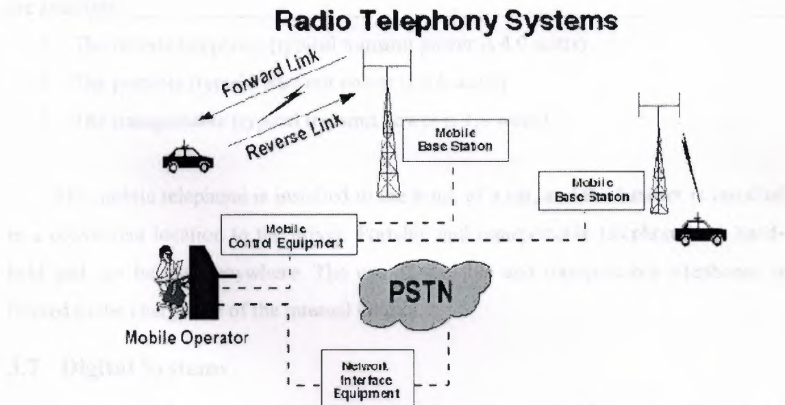
Figure 3.8: Cellular System Components
