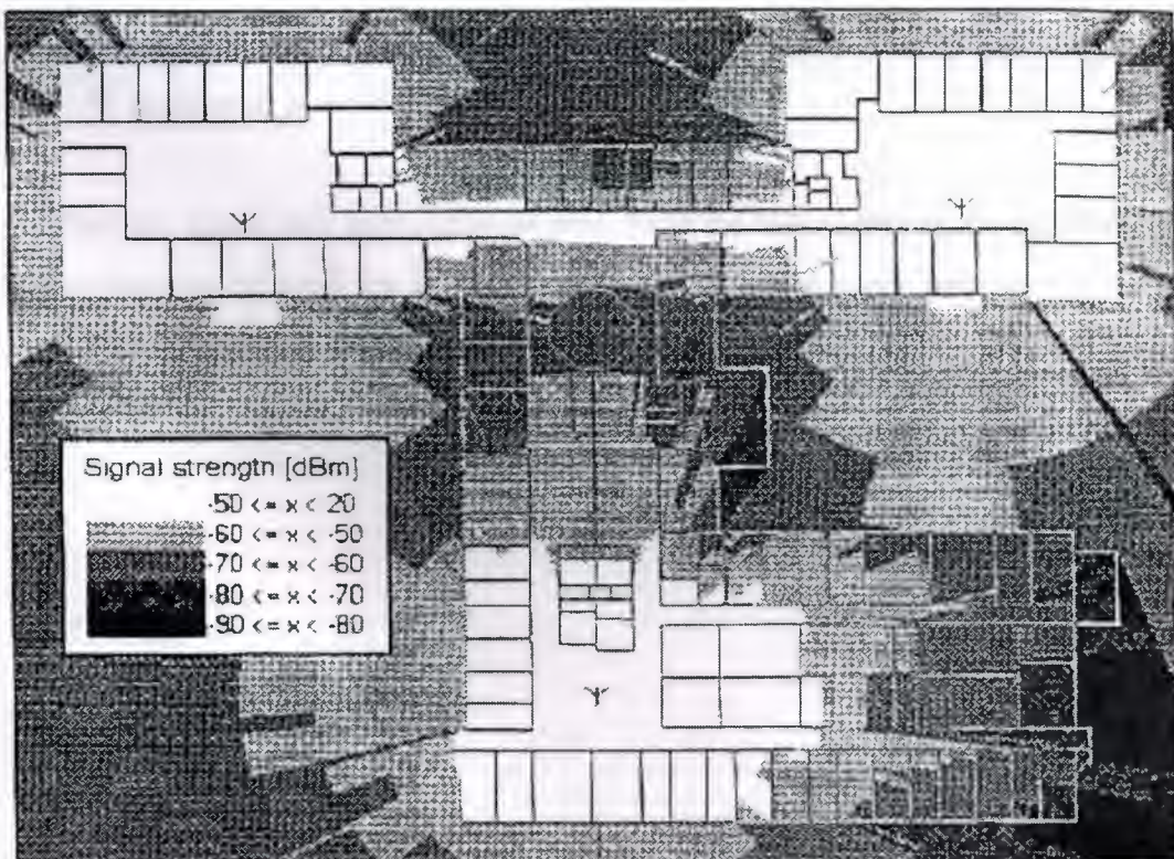
Figure 4.22: Example of signal strength prediction made by TEMS Prediction Omni antennas with 10 dBm EIRP am used
