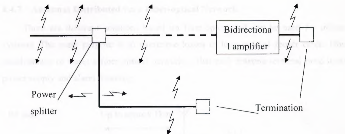
Figure 4.7: Leaking cable.
