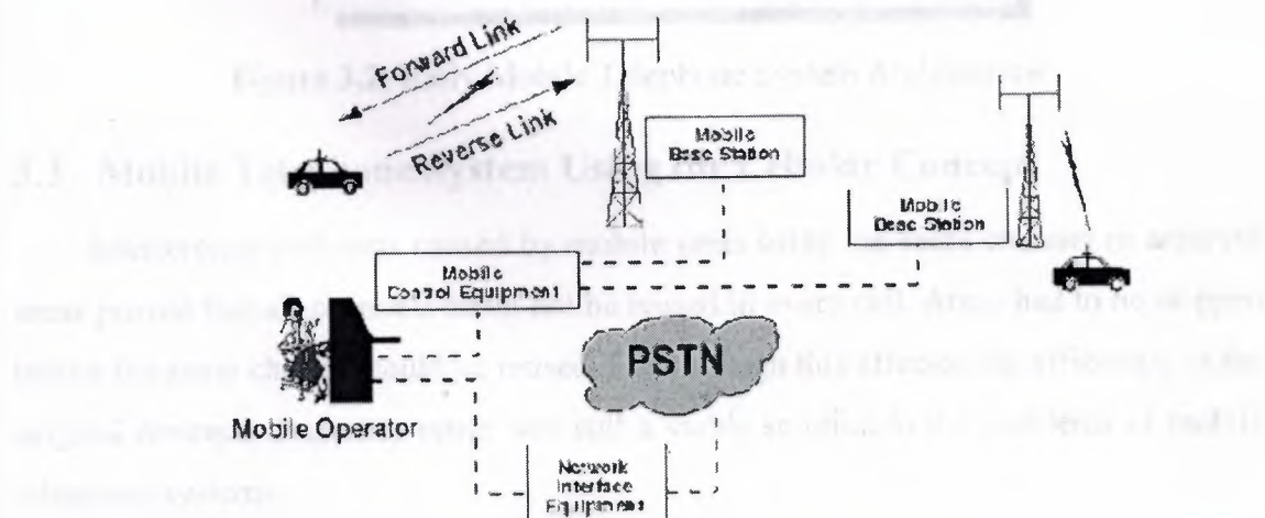
Figure 3.1: Basic Mobile Telephone Service Network
