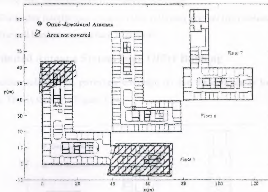
Figure 4.20: Antenna configurations with one antenna.
