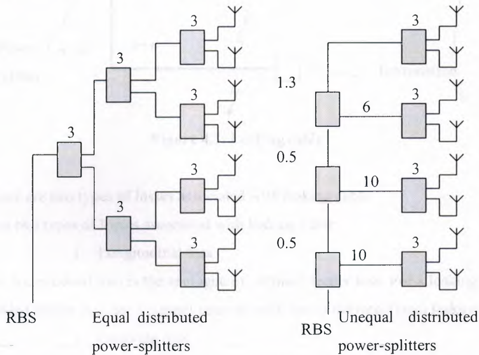
Figure 4.6: Power splitters. Comparison of typical antenna
