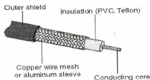
Figure 2.1 Coaxial cable showing various layers
