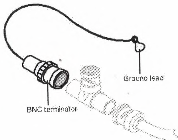
Figure 2.10 BNC terminator
