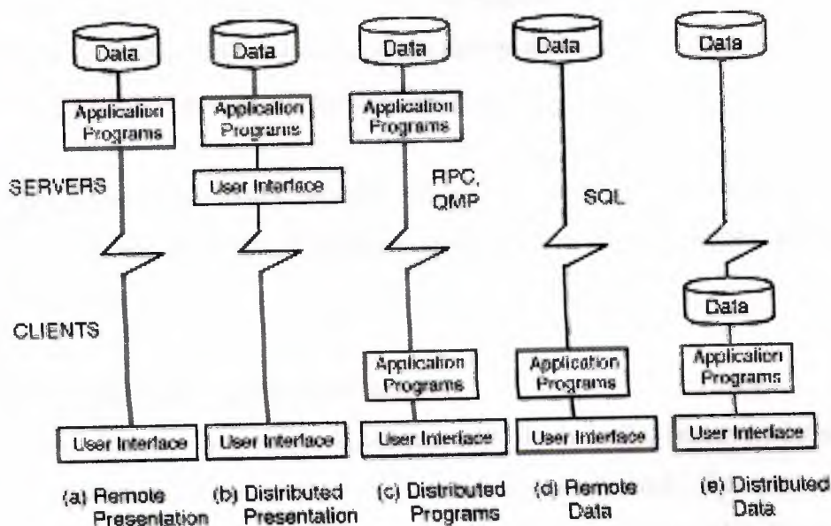
Figure 3.4. Traditional Client/Server Architectures
