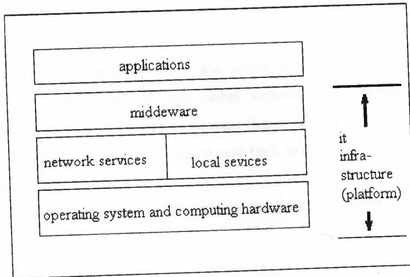
Figure 3.1. Object-Oriented Client/Server Internet Environments
