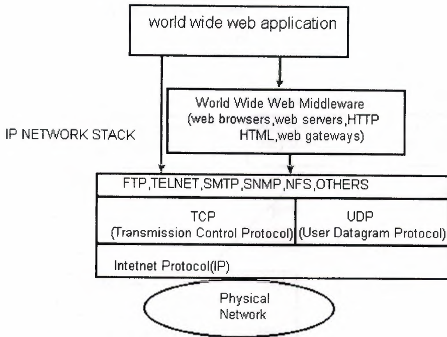
Figure 3.5. Technical View of Internet and World Wide Web
