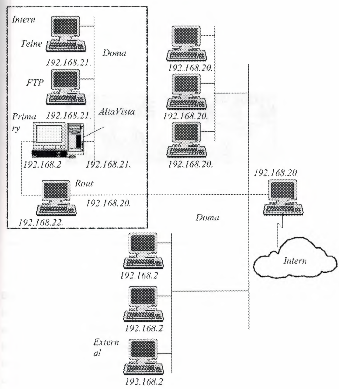
Figure 9.1. Sample Network Configuration with AltaVista Firewall
