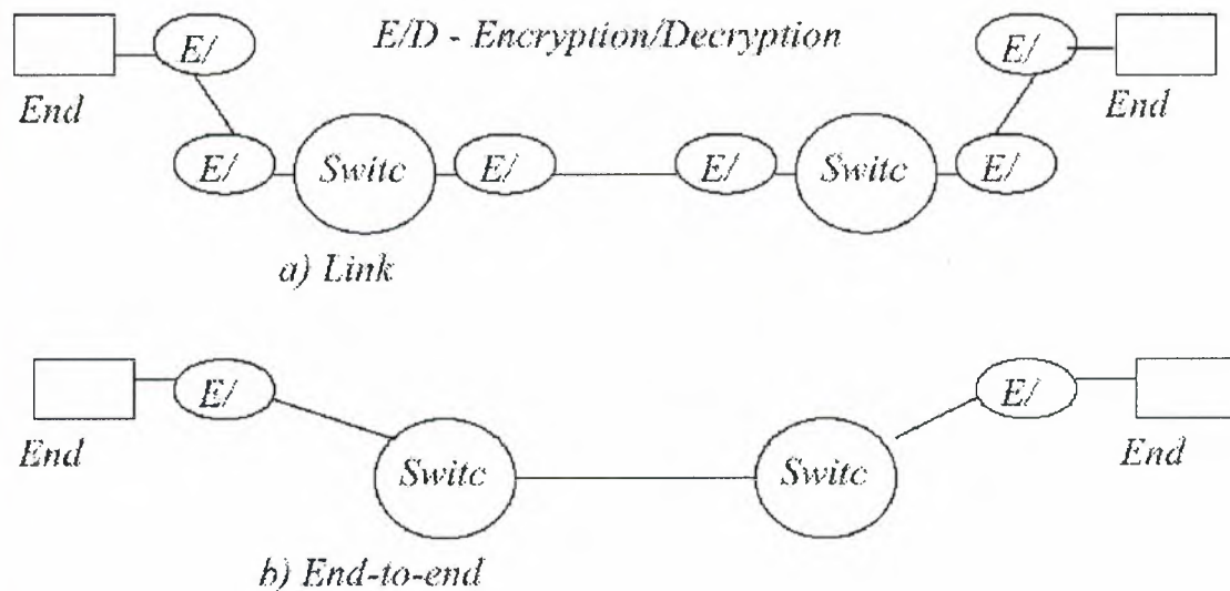
Figure 3.1. Internetwork Encryption
