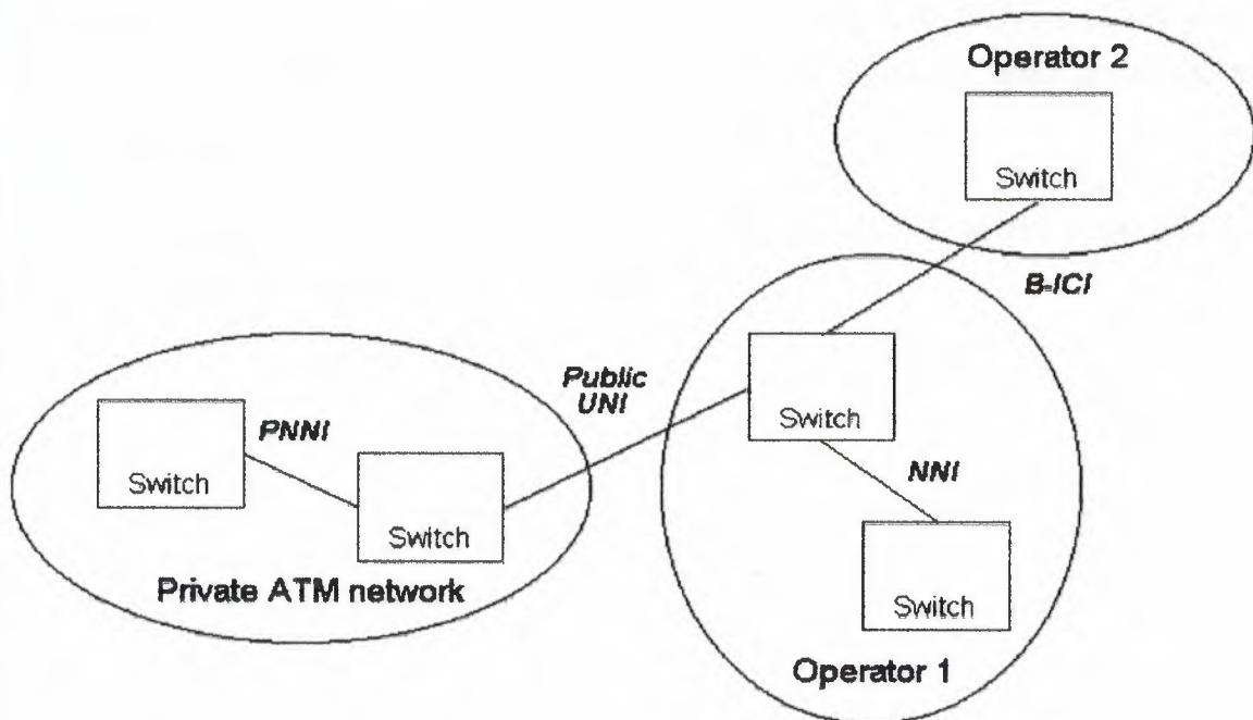
Figure 4.2 ATM network interfaces.
