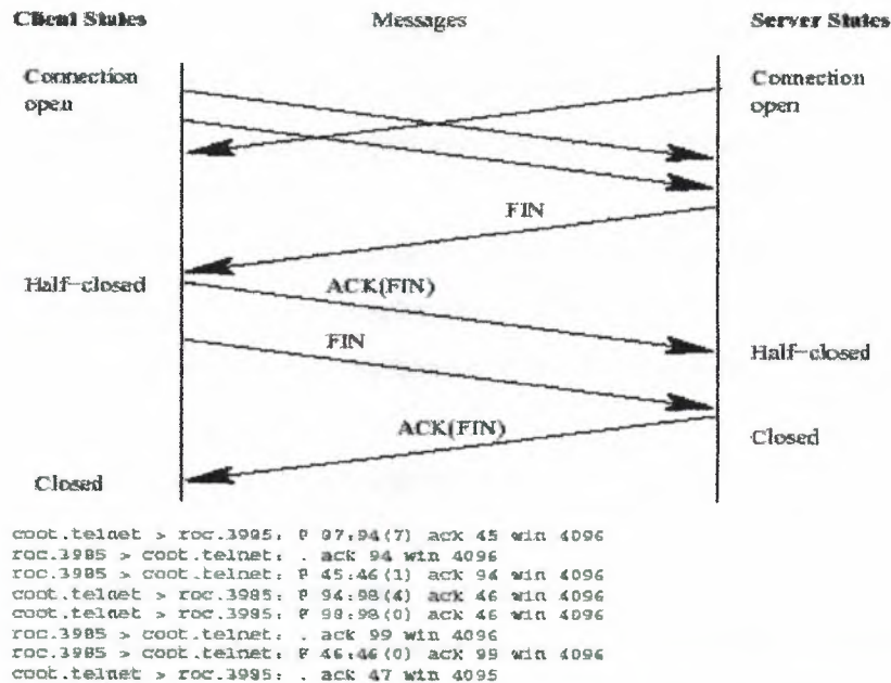
Figure 5.3: TCP I/O The TCP connection is full duplex. Each end sends a FIN packet when it is done transmitting, and the other end acknowledges. (All other packets here contain an ACK showing what has been received; those ACKs are omitted, except for the ACKs of the FINs.) A reset (RST) packet is sent when a protocol violation is detected and the connection needs to be torn down.
