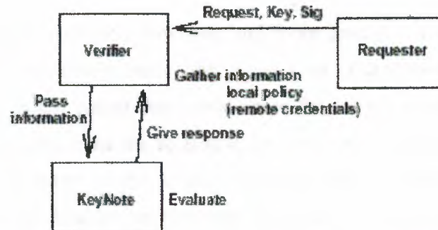
Figure 4.1: Application Interactions with KeyNote. The Requester is typically a user that authenticates through some application-dependent protocol, and optionally provides credentials. The Verifier needs to determine whether the Requester is allowed to perform the requested action. It is responsible for providing to KeyNote all the necessary information, the local policy, and any credentials. It is also responsible for acting upon KeyNote's response.
