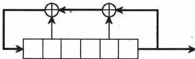
Figure 3.5: Shows a Linear Feed Back Register Model
