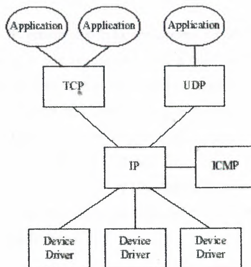
Figure 5.1: A schematic diagram of the different layers involving TCP/IP.
