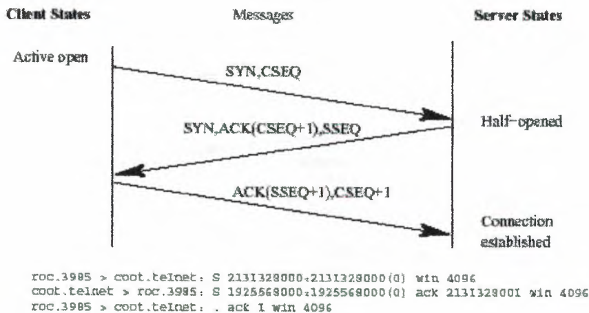
Figure 5.2: TCP Open: The client sends the server a packet with the SYN bit set, and an initial client sequence number CSEQ. The server's reply packet has both the SYN and ACK packets set, and contains both the client's (plus 1) and server's sequence number (SSEQ) for this session. The client increments its sequence number, and replies with the ACK bit set. At this point, either side may send data to the other.
