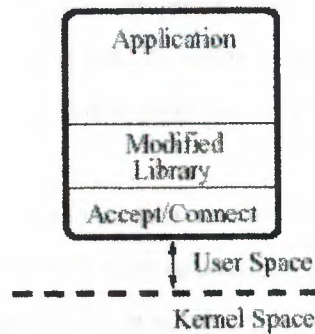
Figure 4.5: Wrappers for filtering the connect(2) and accept(2) system calls are added to a system library. While this approach offers considerable flexibility, it suffers from its inability to guarantee the enforcement of security policies, as applications might not link with the appropriate library.
