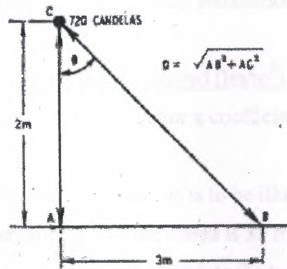
Figure 2.3 Calculating illumination.
