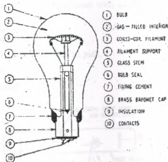
Figure 2.4 Incandescent lamp.
