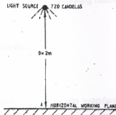
Figure 2.2 Calculating illuminations.
