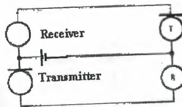
Figure 9.12 Two-position telephone circuit.
