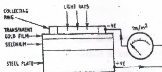
Figure 2.9 Photometer cell.
