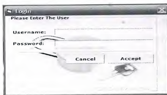
Figure 5.6 Security
