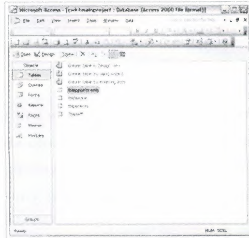
Figure 3.1: MICROSOFT ACCESS
