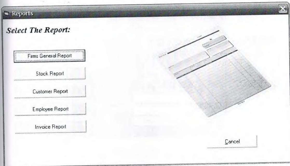
Figure 5.14 Repot
