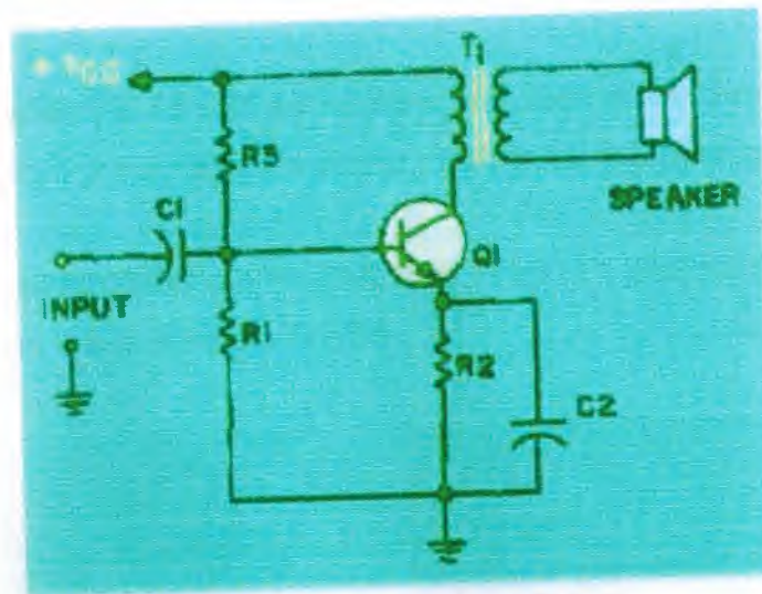
Fig.2.4 Single-stage audio amplifier
