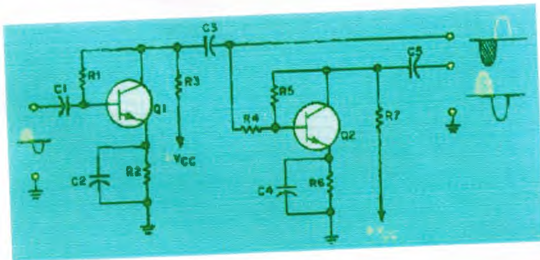
Fig.2.7 Two-stage transistor phase splitter
