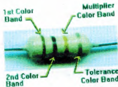
Fig.1.1- Resistor codes
