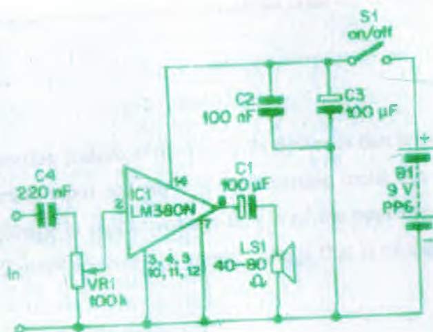
Fig 3.5 the circuit diagram of the simple audio amplifier
