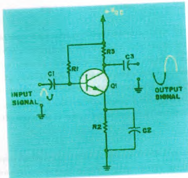
Fig. 2.2 Transistor audio amplifier
