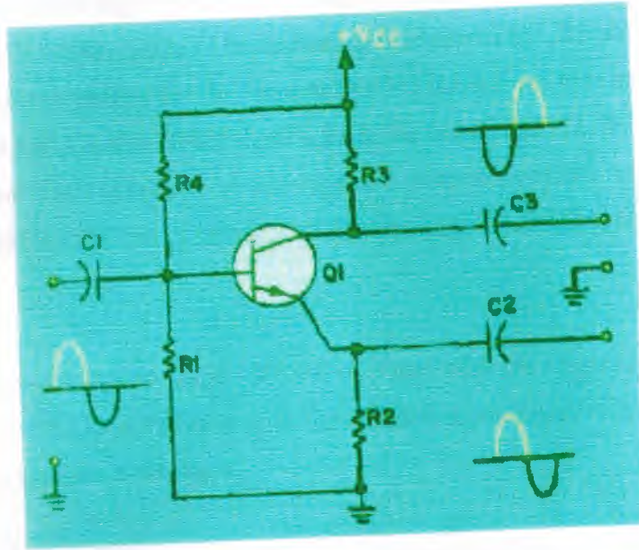
Fig.2.6 Single-stage transistor phase splitter
