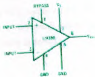
Fig.3.4 LM380N-8
