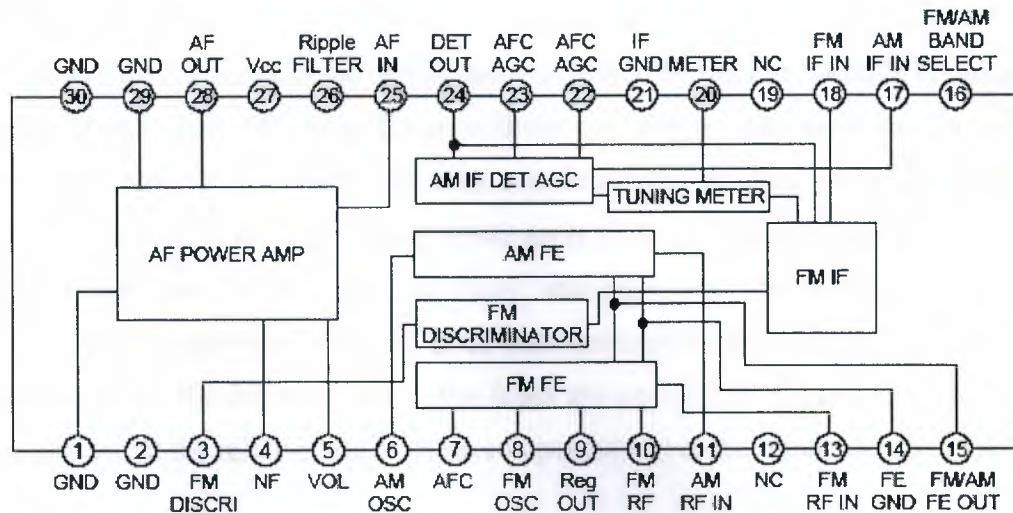
Figure 4.1: Block diagram of CXA1619BS [14]
