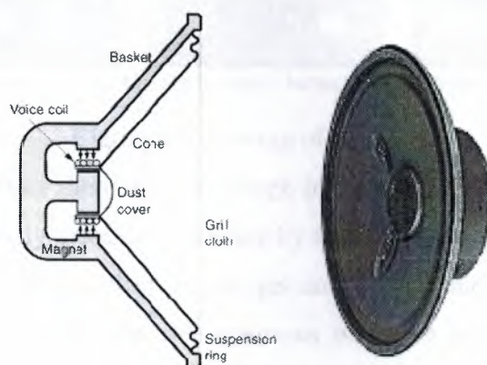
Figure 1.8 Loudspeakers [4]
