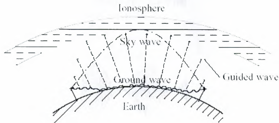
Figure 2.3 Wave propagation [11]
