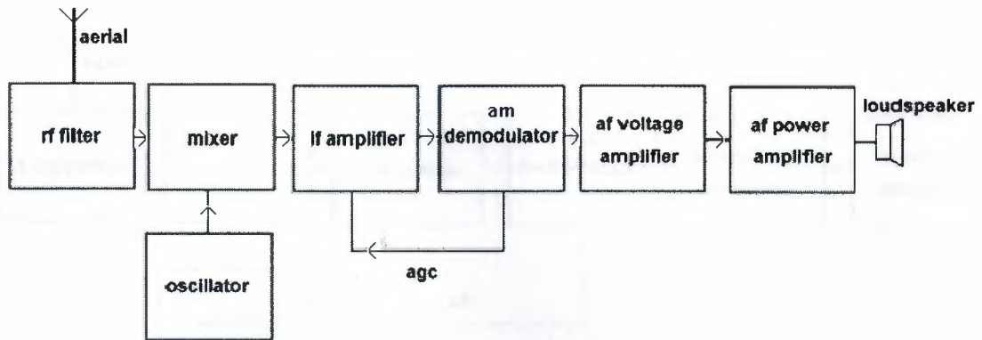
Figure 4.5: AM receiver block diagram [19]
