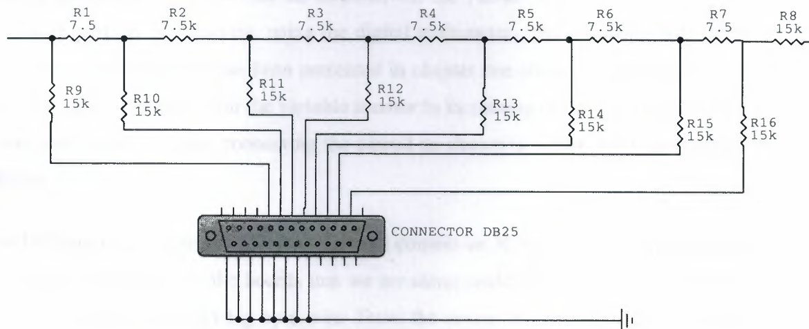
Figure 4.7: Connector DB25 [17]
