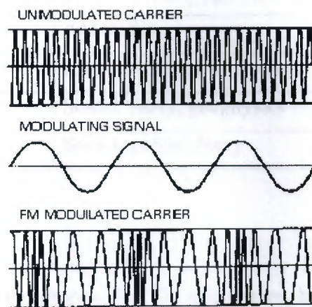
Figure 2.5 Frequency Modulation [12]
