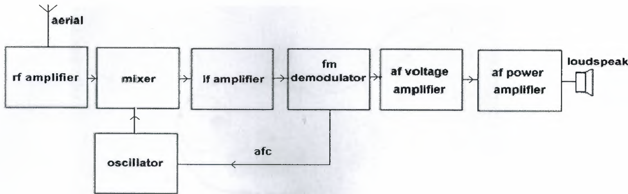
Figure 4.6: FM receiver block diagram [20]
