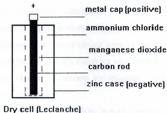
Figure 1.16: Components of the battery
