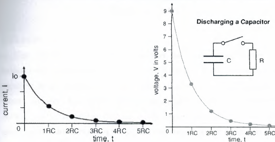
Figure 1.5 Current and voltage for a capacitor discharging [2]
