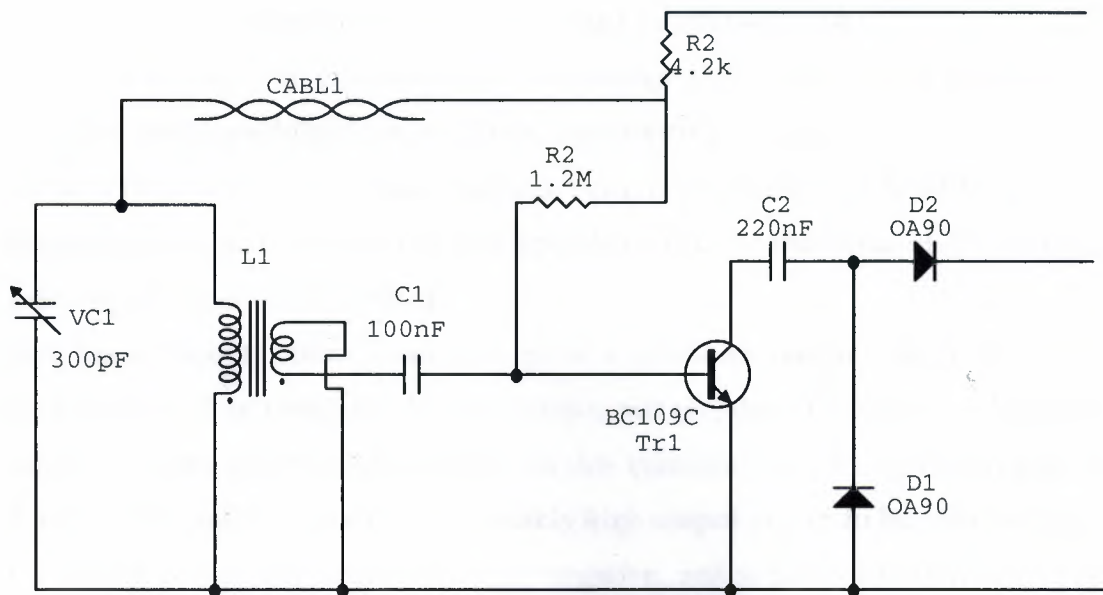
Figure 3.2 Oscillating part diagram of MW radio.
