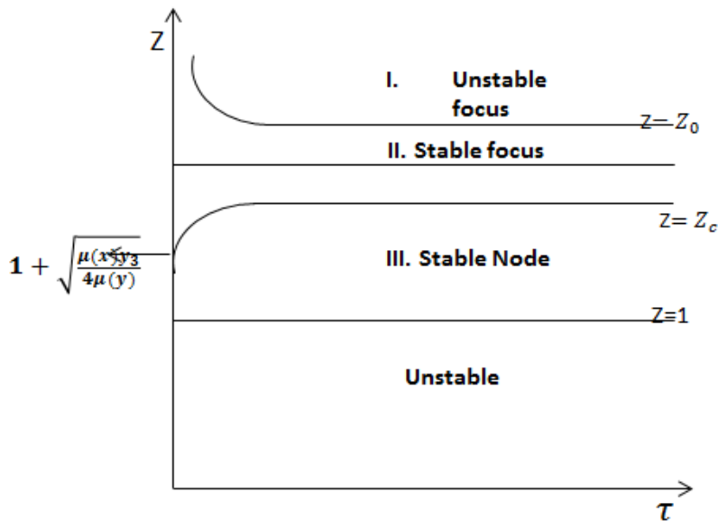
Figure 3.1: : Types of solution for equation 3.13
