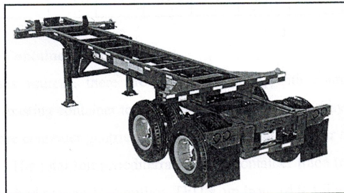
Figure 4.21: Yard Chassis
