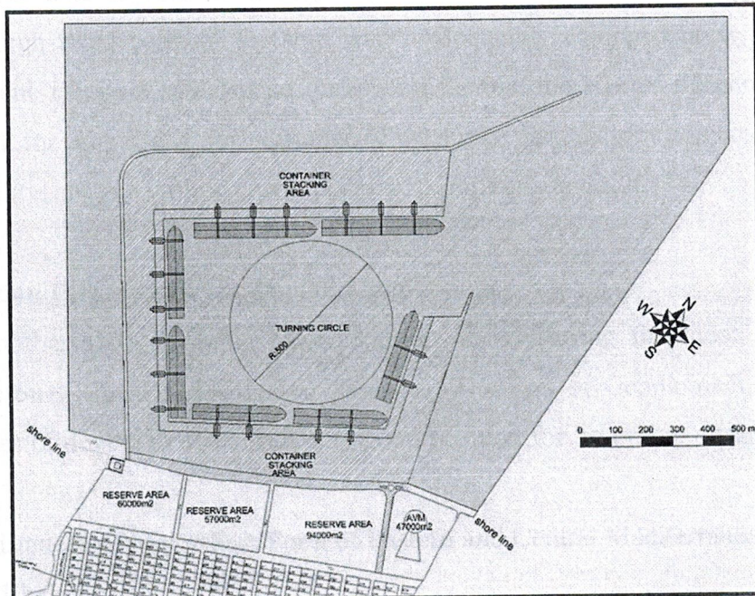
Figure 7.8: Third stage capacity plan of the Port of Gemikona 1 (Port SB 's proposed port of Gemikona 1)
