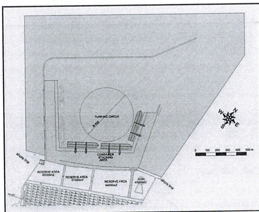
Figure 7.6: First stage capacity plans of the Port of Gemikona 1 (Port SB 's, proposed port of Gemikona 1)
