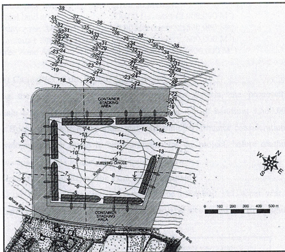
Figure 7.5: Soundings plan of the proposed container terminal at the Port of Gemikona 1 (Port SB 's, proposed container terminal at the Port of Gemikona 1)
