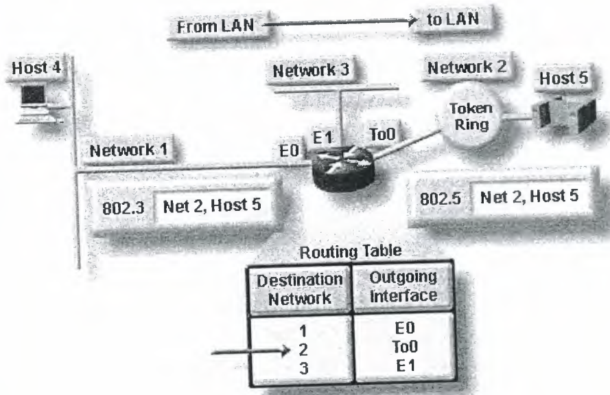
Figure 4.2 Example for LAN-to-LAN routing
