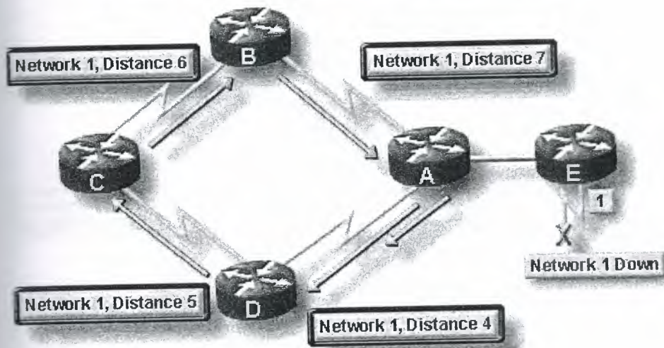
Figure 2.4 Routing Loops Increment The Distance Vector
