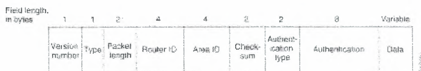
Figure 4.5 OSPF packets consist of nine fields.
