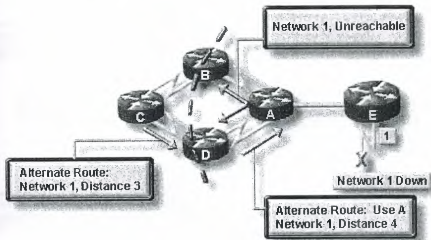
Figure 2.3 Alternative Routes, Slow Convergence, Inconsistent Routing
