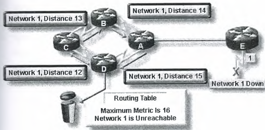
Figure 2.5 Specify a Maximum Distance Vector Metrics As Infinity
