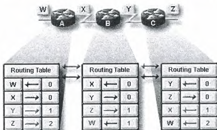
Figure 2.2 Routers Discover the Best Path to Destinations from Each Neighbor
