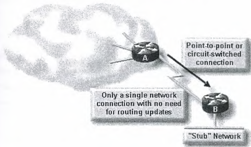
Figure 1-7 Fixed Route To Address Reflects Administrator's Knowledge
