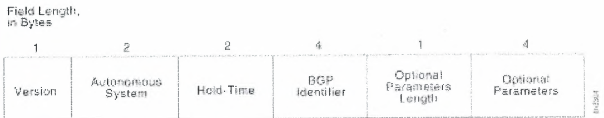
Figure 4.11: A BGP open message consists of six fields.
