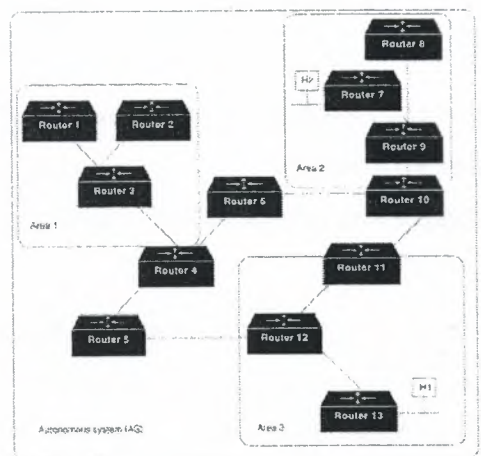
Figure 4.4: An OSPF AS consists of multiple areas linked by routers In the figure
