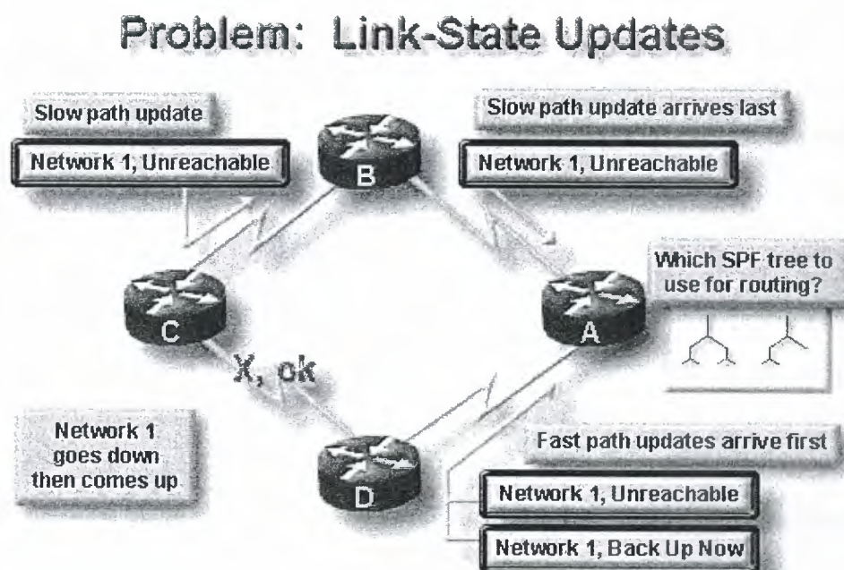
Figure 3.1 Unsynchronized Updates, Inconsistent Path Decision
