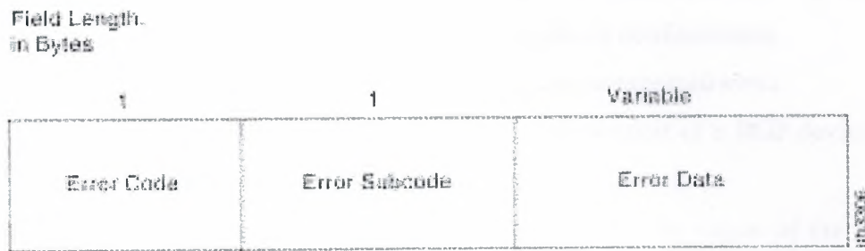
Figure 4.13 A BGP notification message consists of three fields.
