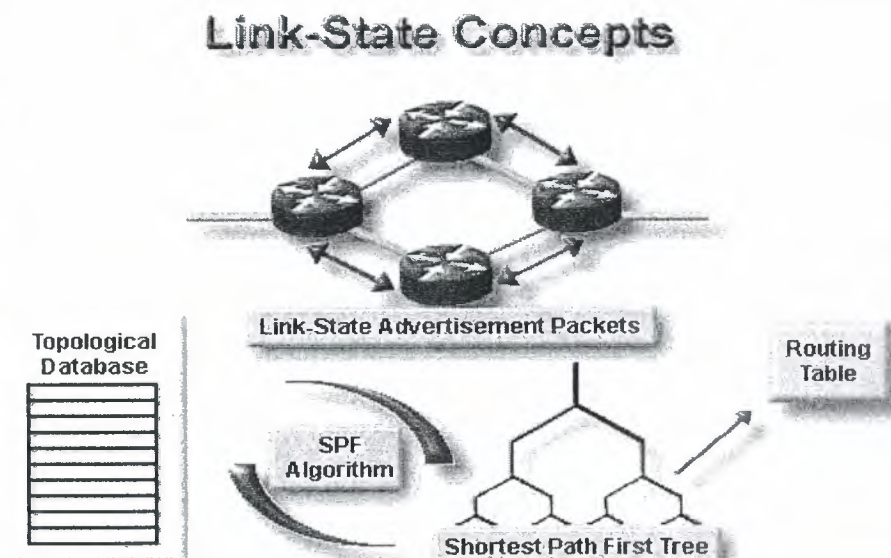
Figure 2.8 After Initial flood, pass Small Event-triggered Link-State Updates to All Other Router
