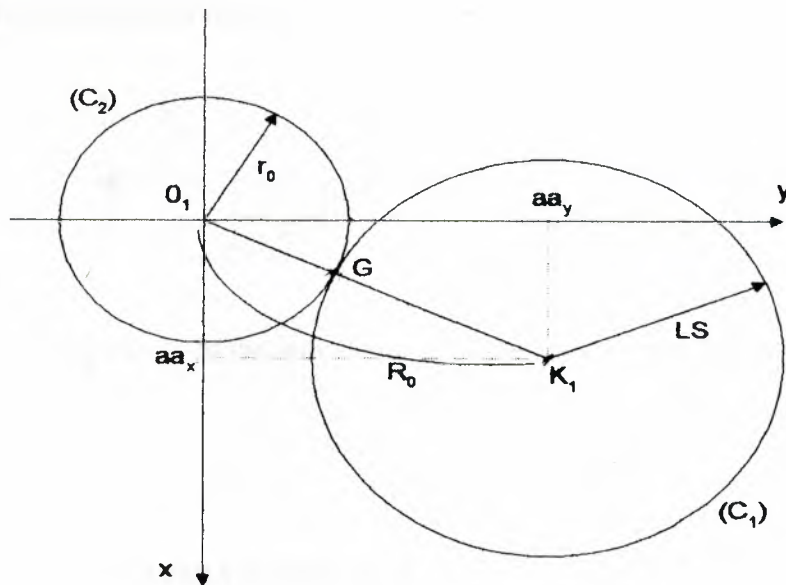
Fig 3.6 Geometry for the location of Gin II plane
