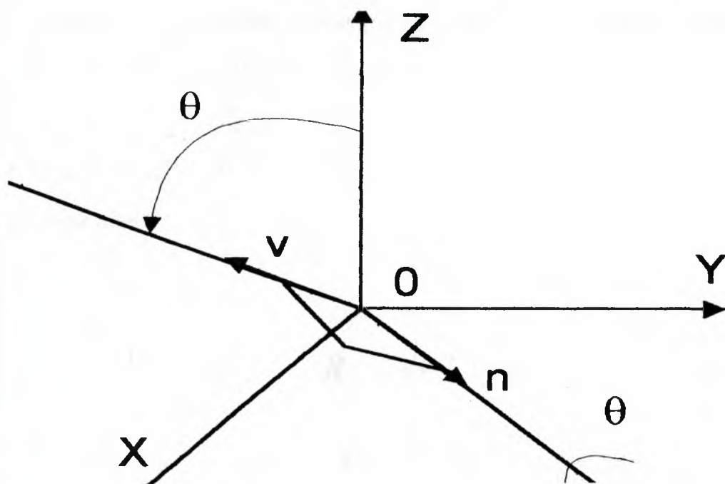
Fig 3.4 Interpretation of the transformation
