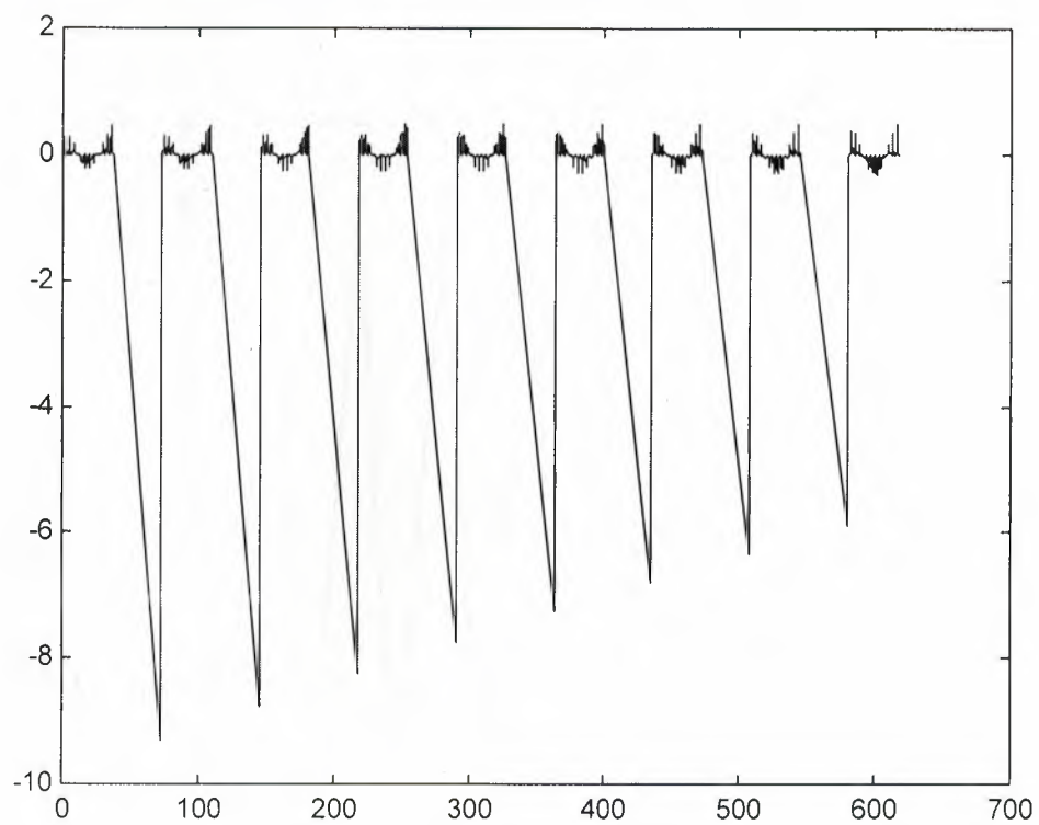
Fig 3.9 Shows the velocity of the extendible limb Plot ( \dot{l} , t )
