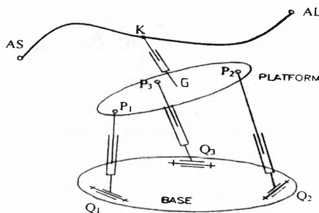
Fig 3.1 4-DOF Stewart Platform
