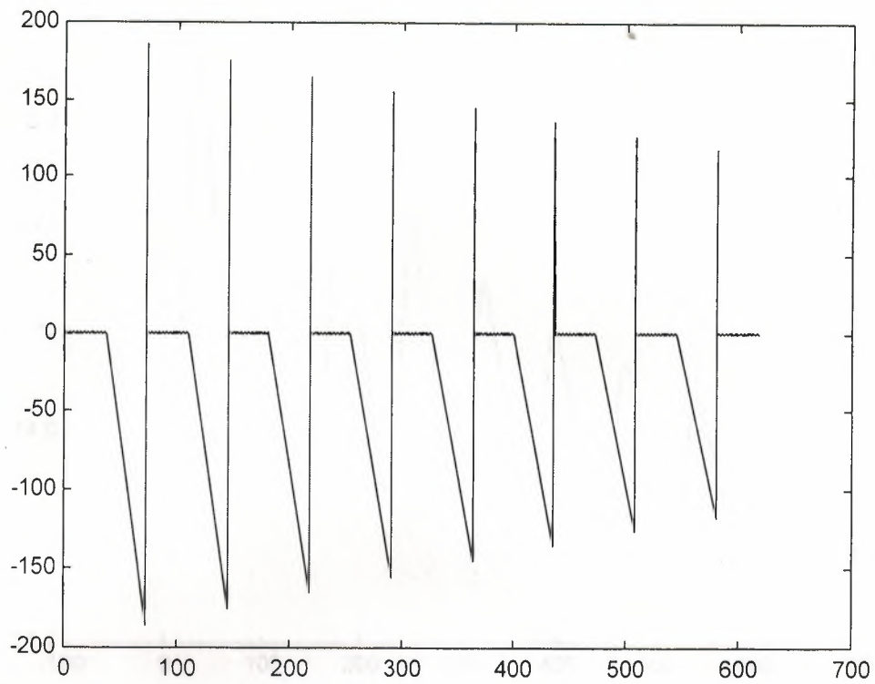
Fig 3.9 Shows the acceleration of the extendible limb Plot (ltti,lli)
