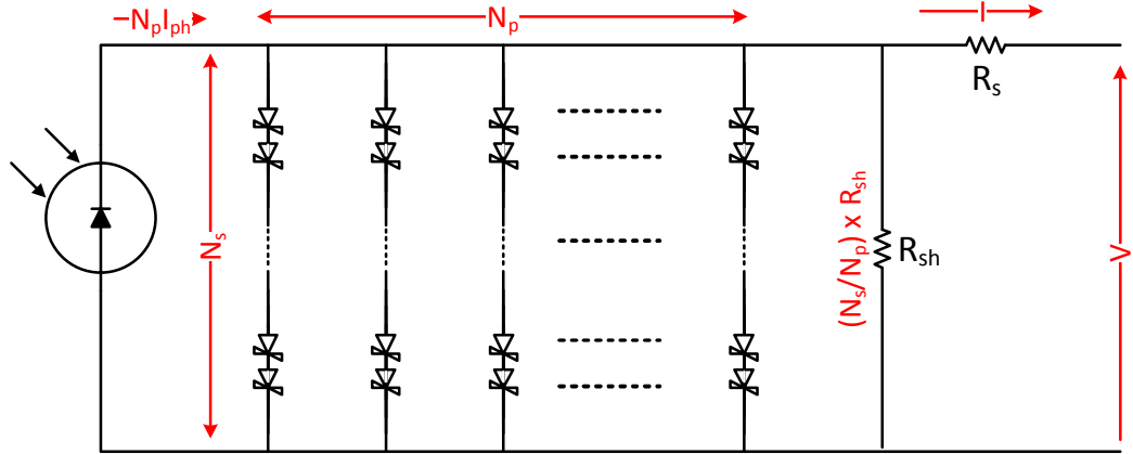
Figure 8: General model of an equivalent PV array
