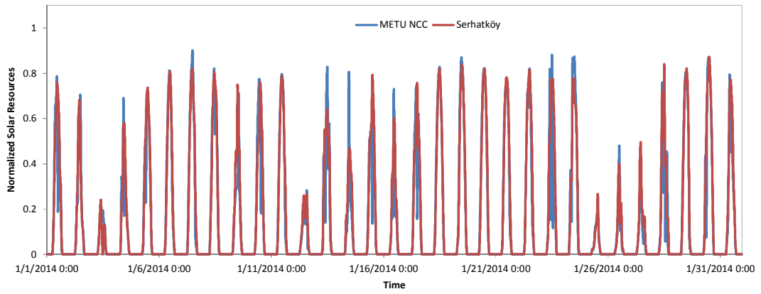
Figure A 8 :Comparison between Normalized METU NCC and Serhatköy Solar Resource Data for January 2014 [29]
