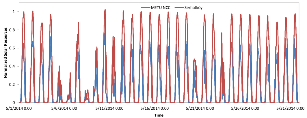
Figure A 12 :Comparison between Normalized METU NCC and Serhatköy Solar Resource Data for May 2014 [29]
