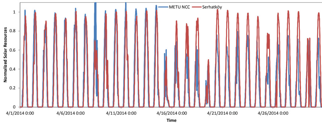
Figure A 11 :Comparison between Normalized METU NCC and Serhatköy Solar Resource Data for April 2014 [29]
