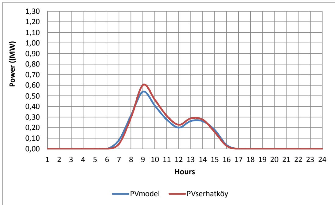
Figure 25: Serhatkőy Electricity Generation vs PVmodel output in Winter Solstice, 21 st December 2013
