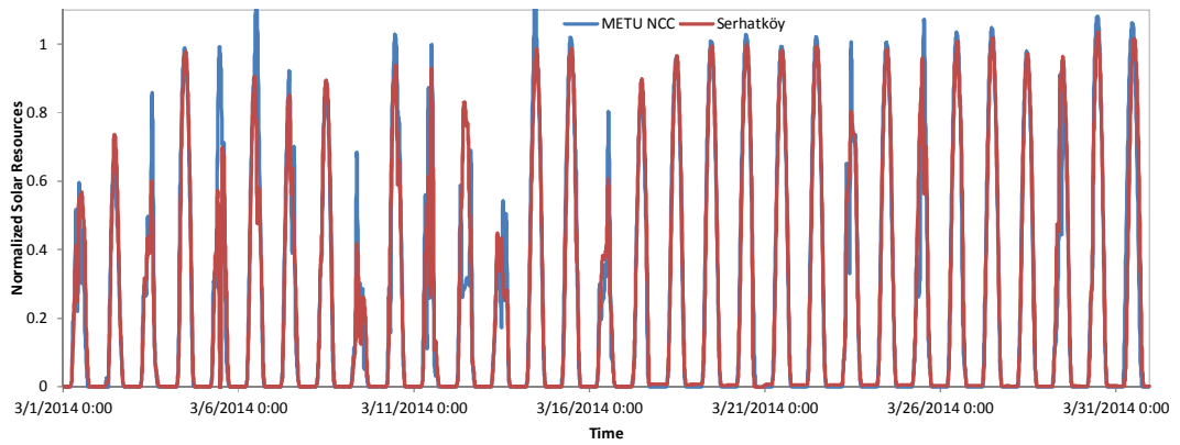
Figure A 10 :Comparison between Normalized METU NCC and Serhatköy Solar Resource Data for March 2014 [29]
