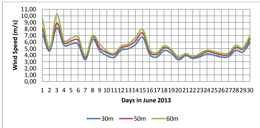
Figure 16: Average daily wind speed distribution in June 2013
