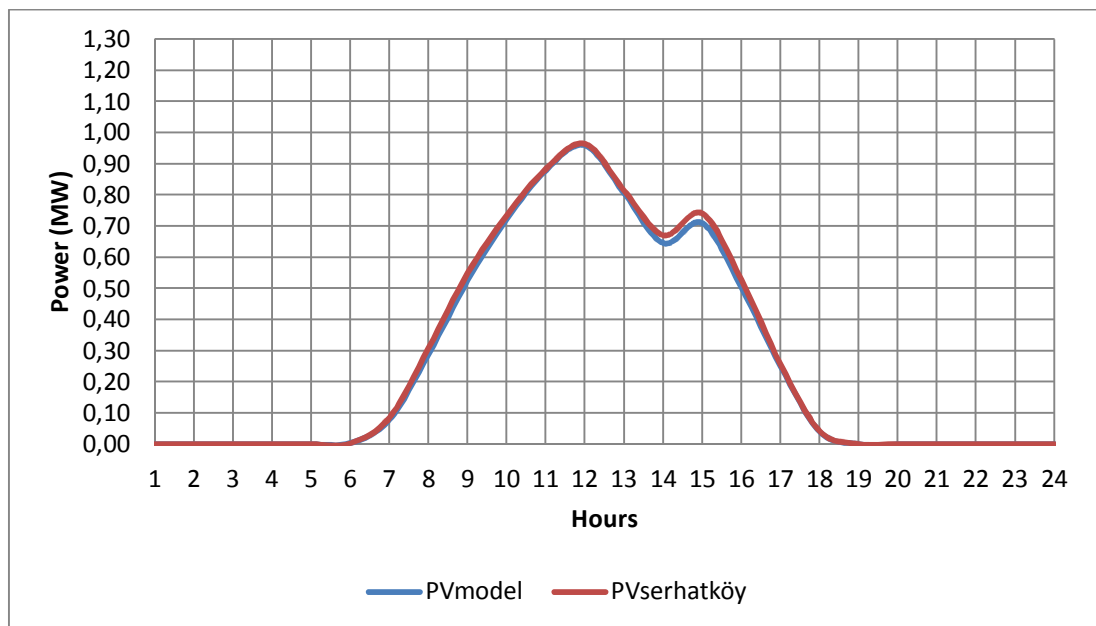
Figure 24: Serhatkőy Electricity Generation vs PVmodel output in Fall Equinox, 21 st September 2013
