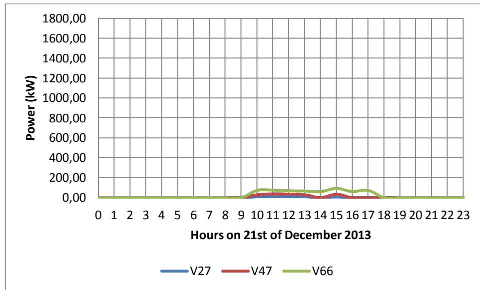
Figure 35: Vestas V27, V47, V66 electricity generation prediction model output on 21 st of December 2013
