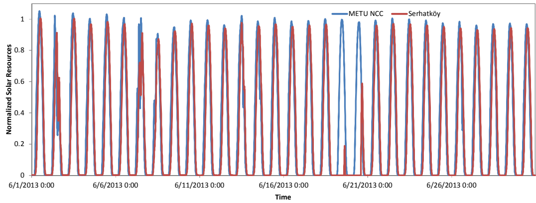
Figure A 1 :Comparison between Normalized METU NCC and Serhatköy Solar Resource Data for June 2013 [29]
