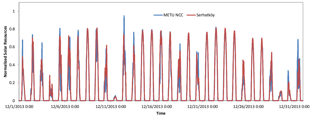
Figure A 7 :Comparison between Normalized METU NCC and Serhatköy Solar Resource Data for December 2013 [29]
