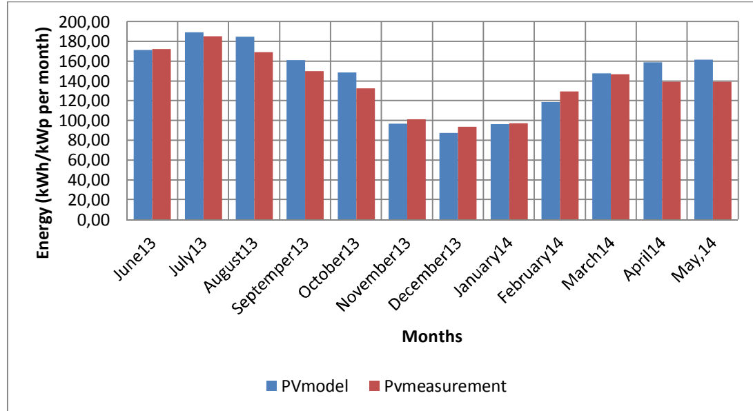
Figure 27: PVmodel vs Serhatköy Measurement normalized to 1 kW p
