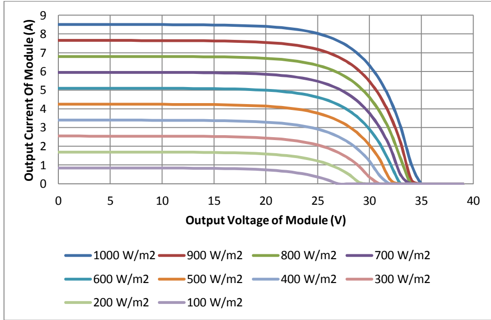
Figure 11: I-V curve of the proposed PV model under different solar irradiation condition
