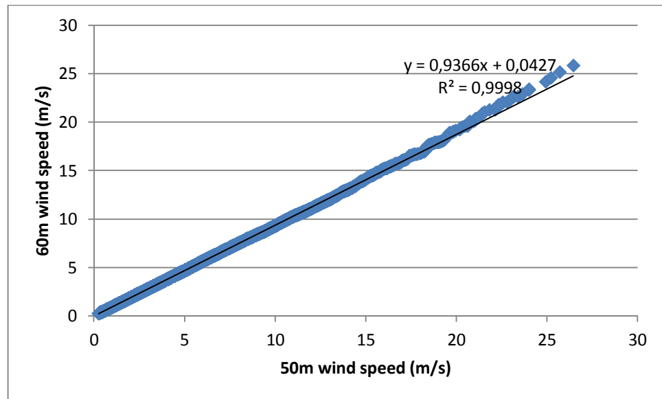
Figure 18: 60 meter and 50 meter wind correlation
