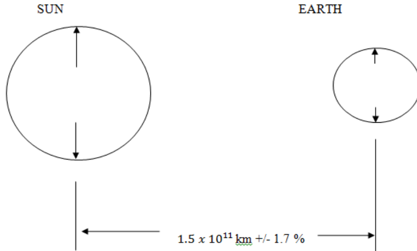
Figure 13: Distance between the Sun and Earth
