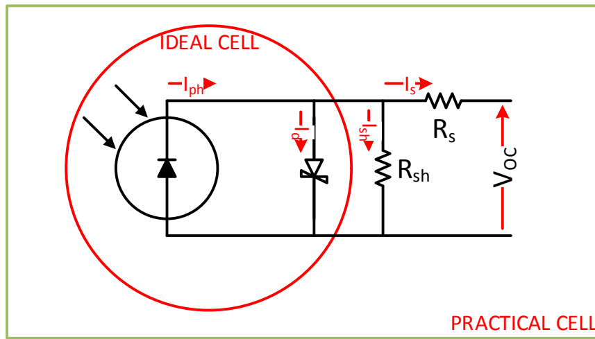
Figure 7: General model of a PV cell/module in a single diode model
