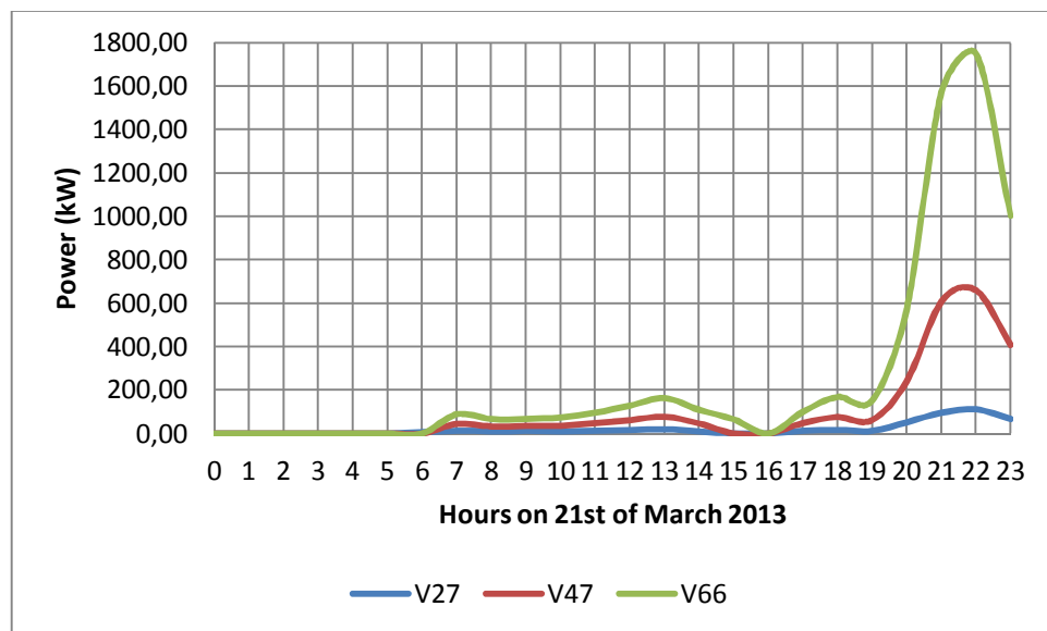
Figure 32: Vestas V27, V47, V66 electricity generation prediction model output on 21 st of March 2013
