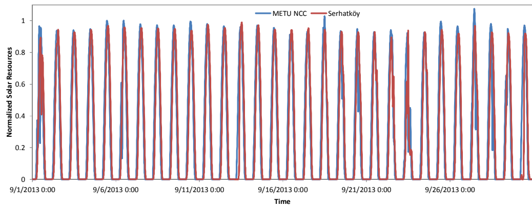
Figure A 4 :Comparison between Normalized METU NCC and Serhatköy Solar Resource Data for September 2013 [29]
