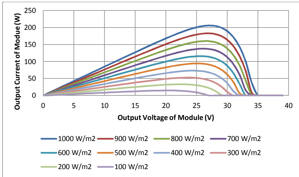
Figure 12: P-V curve of the proposed PV model under different solar irradiation condition
