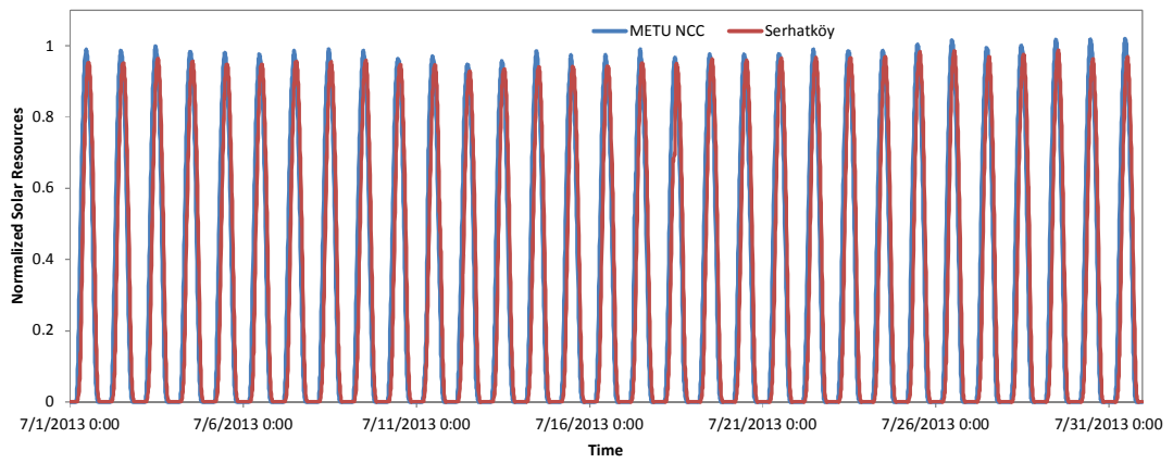
Figure A 2 :Comparison between Normalized METU NCC and Serhatköy Solar Resource Data for July 2013 [29]
