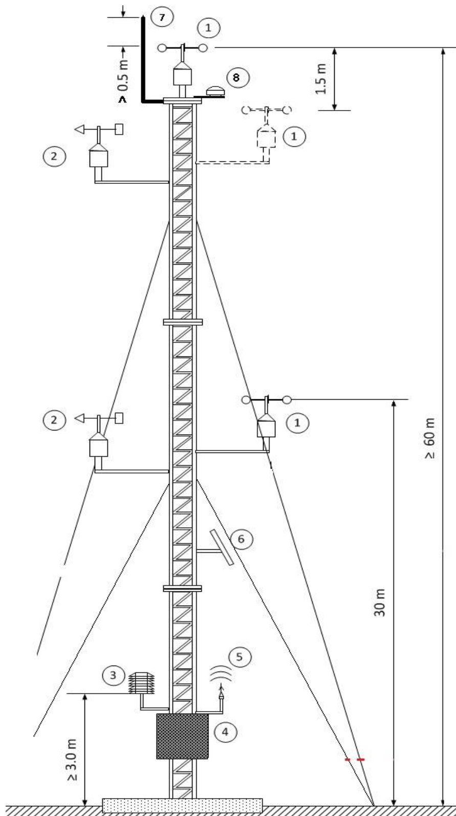
Figure 14: Wind Tower Model
