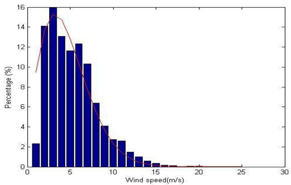
Figure 31: 60m weibull analysis
