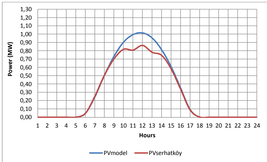
Figure 26: Serhatkőy Electricity Generation vs PVmodel output in Fall Equinox, 21 st March 2014
