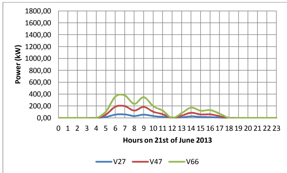
Figure 33: Vestas V27, V47, V66 electricity generation prediction model output on 21 st of June 2013
