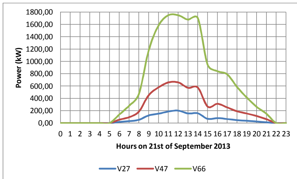
Figure 34: Vestas V27, V47, V66 electricity generation prediction model output on 21 st of September 2013
