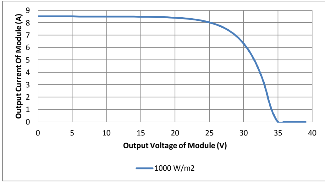
Figure 9: I-V curve of the proposed PV model under standard test conditions
