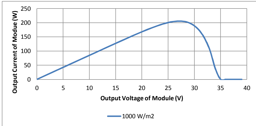
Figure 10: P-V curve of the proposed PV model under standard test conditions
