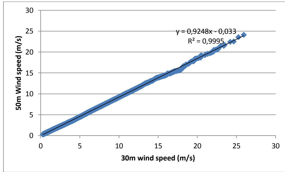
Figure 20: 50 meter and 40 meter wind correlation
