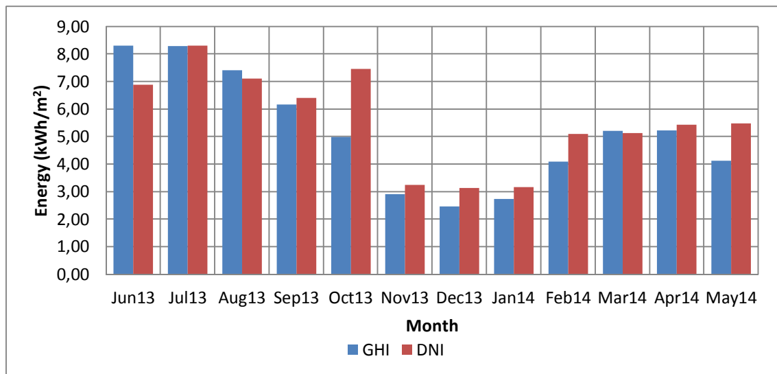
Figure 2: Monthly average global horizontal and direct normal solar irradiation
