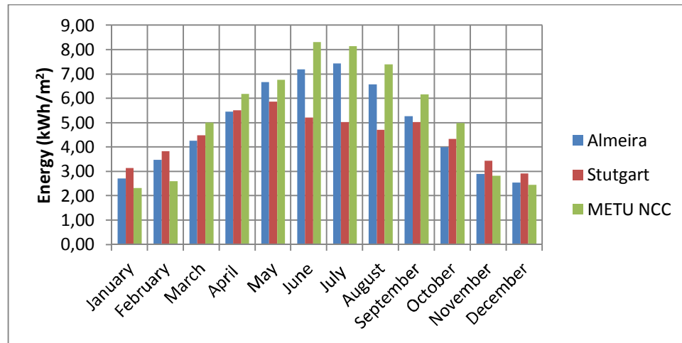
Figure 28: Average monthly global horizontal solar irradiation measurements in Almeria, Stuttgart and MET U NCC in 2013 [55]
