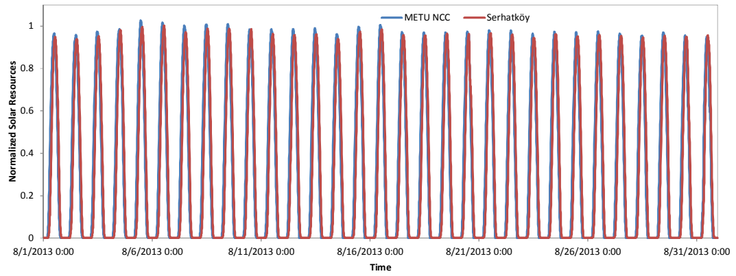
Figure A 3 :Comparison between Normalized METU NCC and Serhatköy Solar Resource Data for August 2013 [29]
