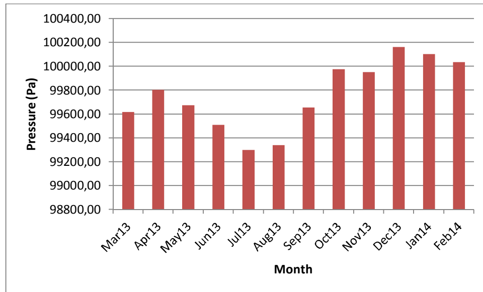
Figure 21: METU NCC Wind tower monthly average pressure
