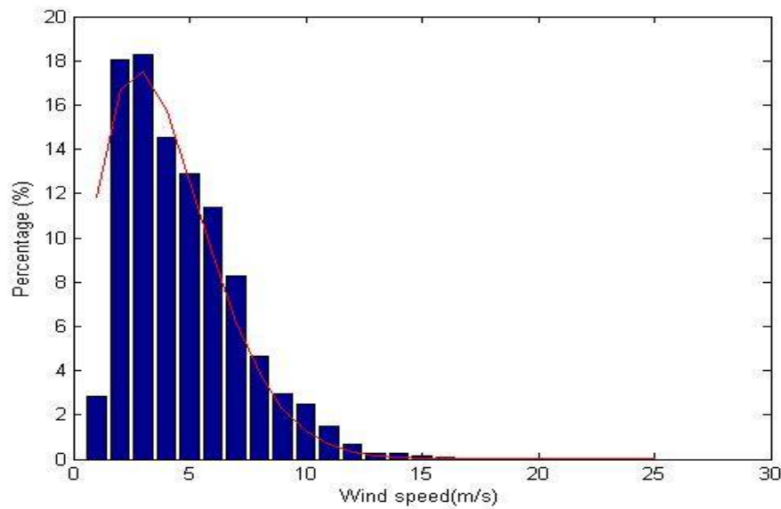
Figure 29: 30m weibull analysis
