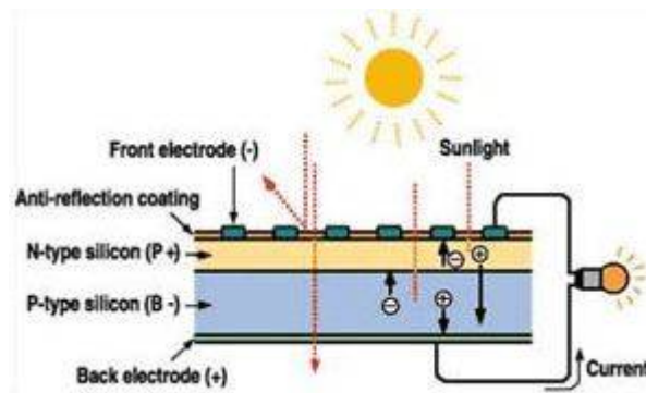
Figure 5: P-N junction illustration of Photovoltaic Cell [37]
