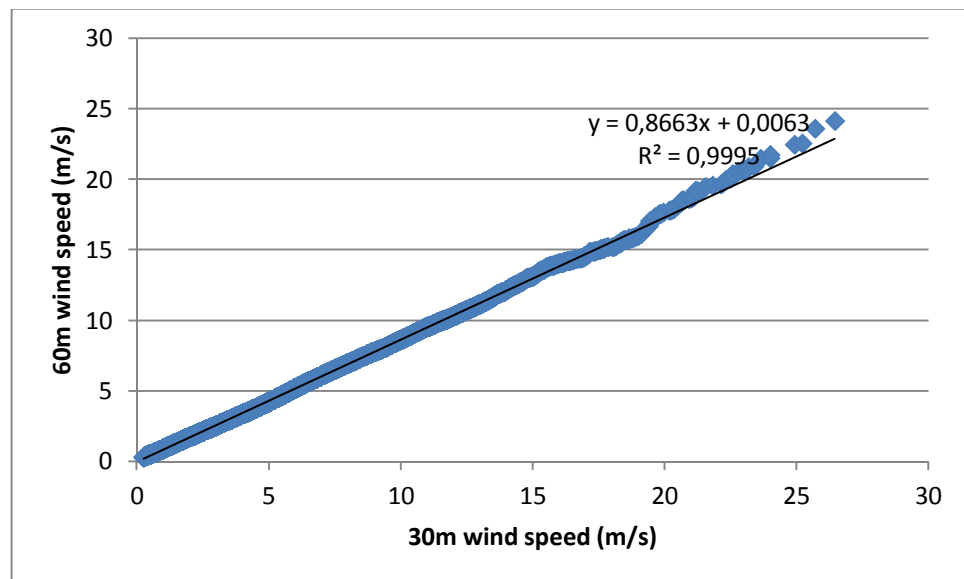
Figure 19: 60 meter and 30 meter wind correlation
