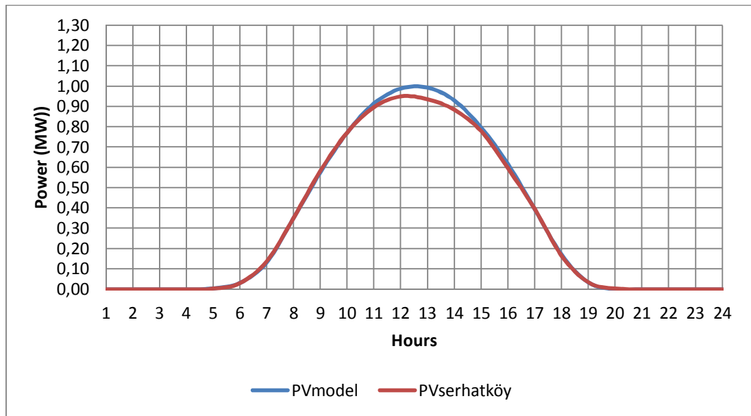
Figure 23: Serhatkőy Electricity Generation vs PVmodel output in Summer Solstice, 21 st June 2013
