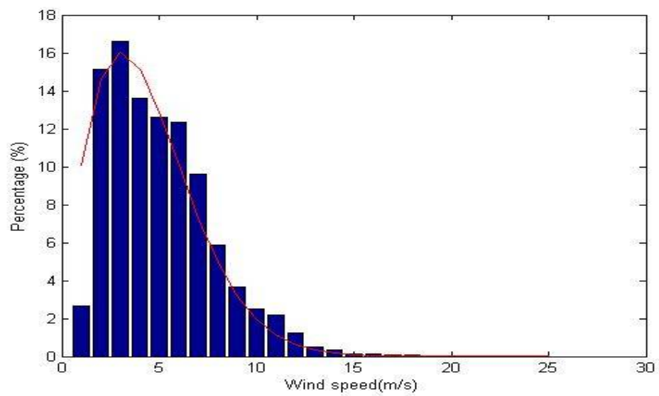
Figure 30: 50m weibull analysis
