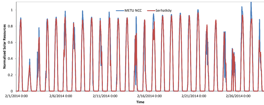
Figure A 9 :Comparison between Normalized METU NCC and Serhatköy Solar Resource Data for February 2014 [29]
